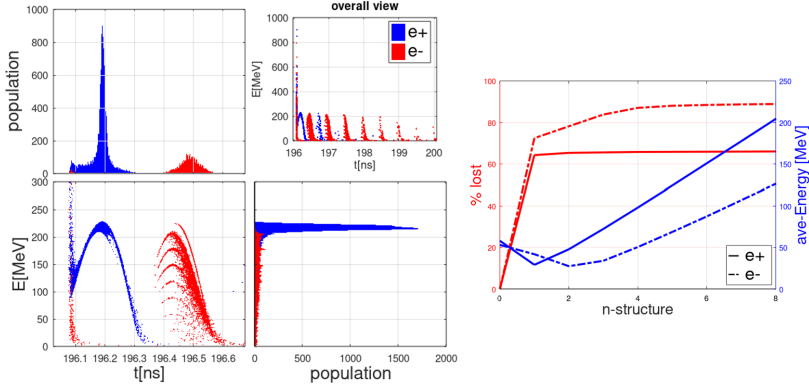
Figure 4. left : Longitudinal phase-space for electrons (red) and positrons (blue) without Beam Loading consideration. right: Average energy and loss percentage
