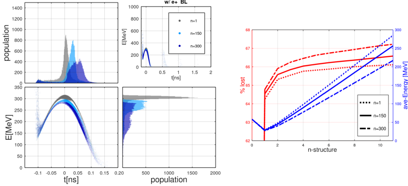
Figure 6. left: Longitudinal phase-space right: Average energy and loss percentage for positrons considering positron Beam Loading. Results are shown for the first, middle, and one of last bunches in the train, (the deceleration phase applied in the first structure and acceleration phases in the subsequent structures.)
