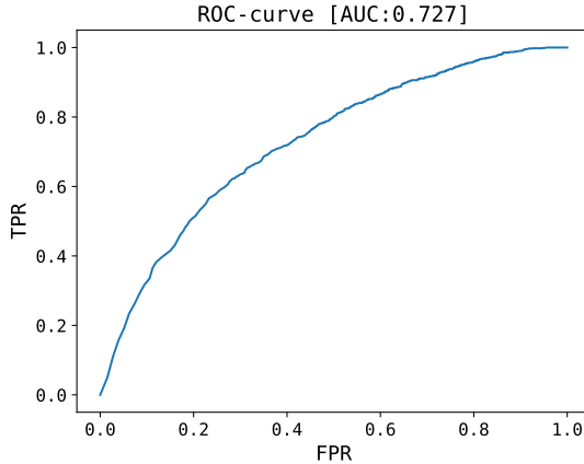
Figure 8: ROC-curve of the ZHH/ZZH discriminator using the full MEM procedure.
