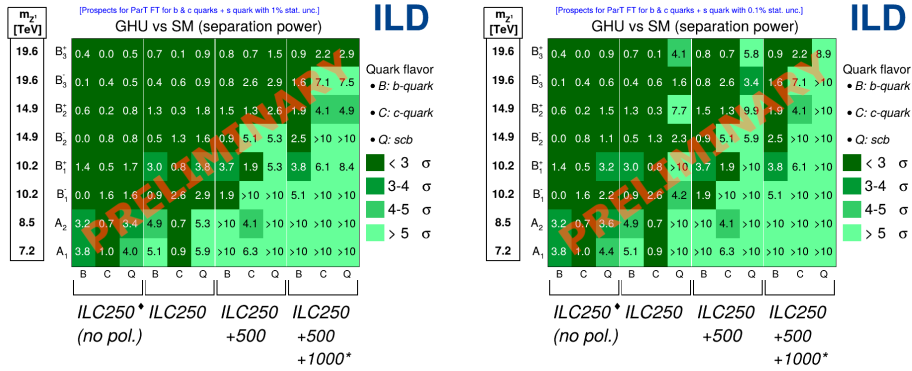
Fig. 5 Expected impact in the discrimination power for GHU models assuming a 1% (left) or 0.1% (right) uncertainty for s\bar{s} .
