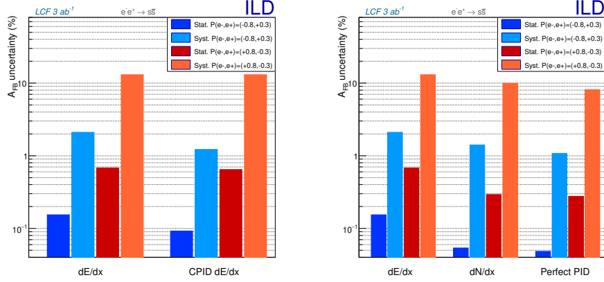
Fig. 4 Expected uncertainties for s\bar{s} in the LCF@CERN250. Left: Comparing different software approaches ( dE/dx vs CPID dE/dx ). Right: Comparing different hardware settings ( dE/dx vs dN/dx in a pixel TPC vs An ideal TPC)
