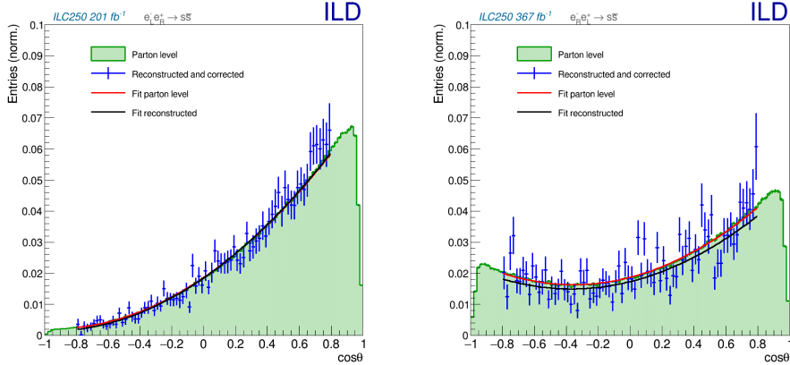
Fig. 2 Comparison of the angular fits to the reconstructed and corrected data with respect to the parton level distributions. Plots for the e_L^- e_R^+ (left) and e_R^- e_L^+ (right) cases using dE/dx .
