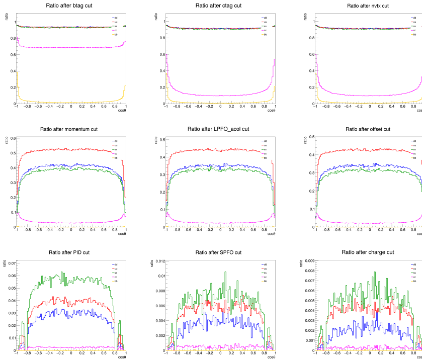
Fig. A2 Efficiencies per cut in the e_R^- e_L^+ case.
