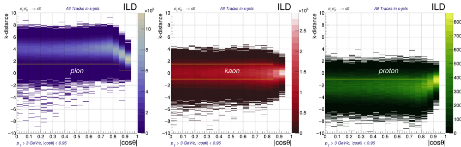
Fig. 1 Kaon selection region in the k -distance plane used in cut 7.
