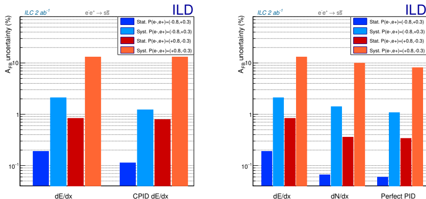
Fig. 3 Expected uncertainties for s\bar{s} in the ILC250. Right: Comparing different hardware settings ( dE/dx vs dN/dx in a pixel TPC vs An ideal TPC)
