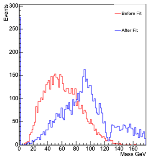
Z Mass
