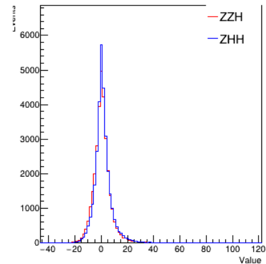
Jet Energy Pull
