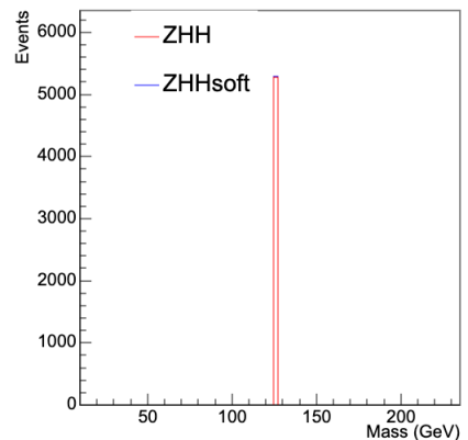
H2 Mass
