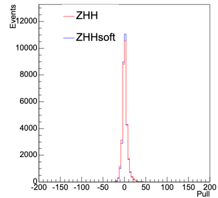
Jet Energy Pull
