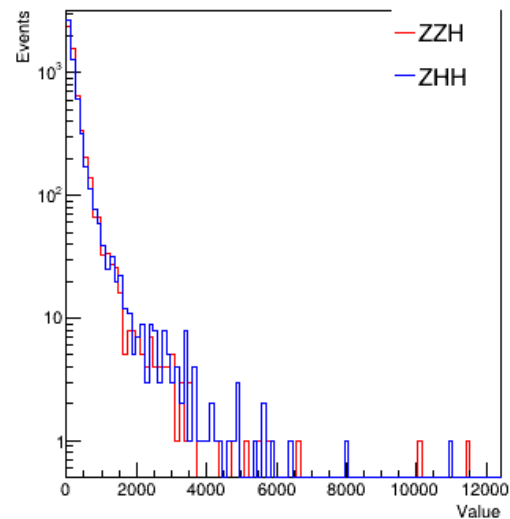
ZHH Mass
