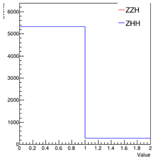
Z Mass
