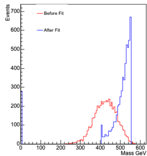
ZHH Mass
