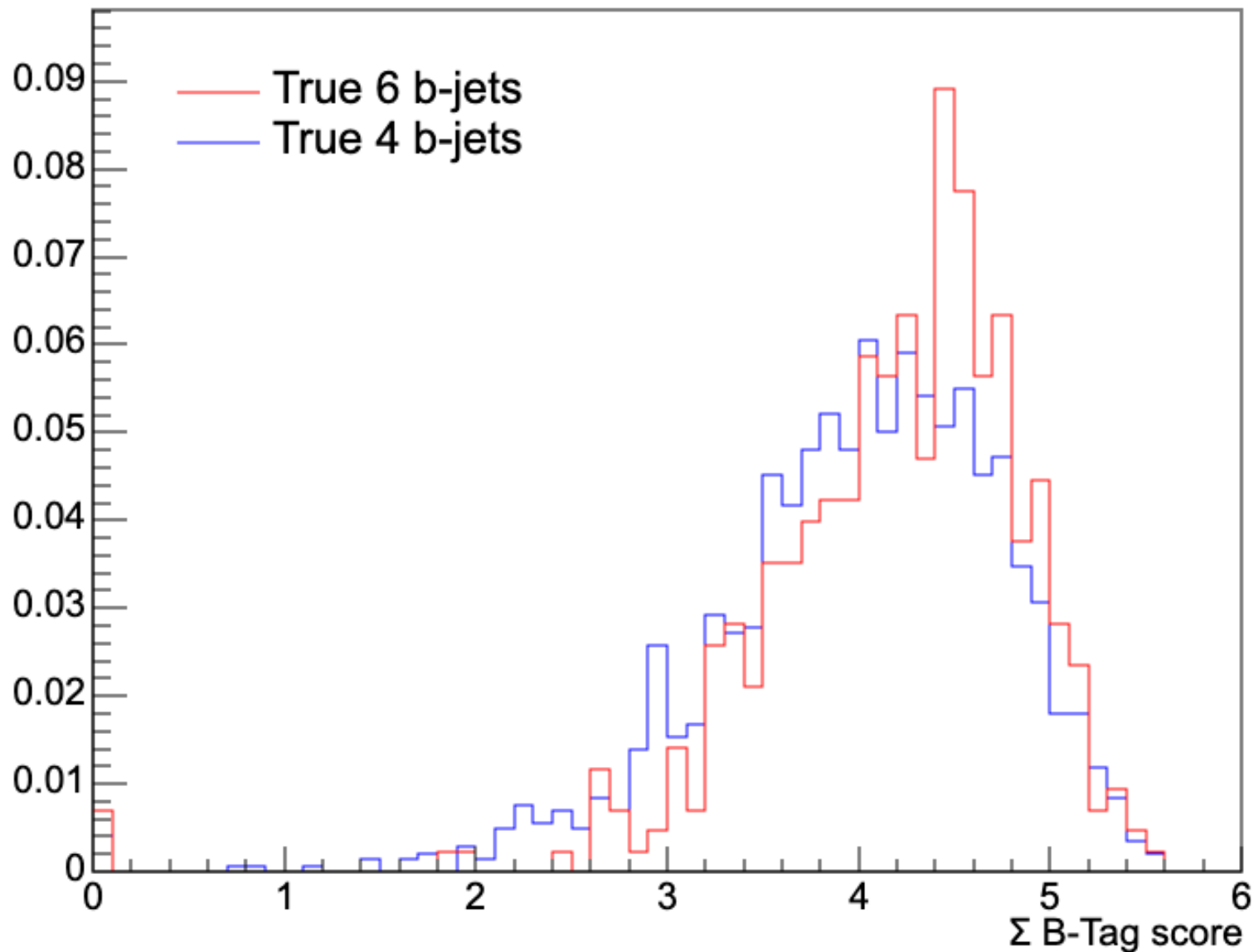
Sum of B-Tags
