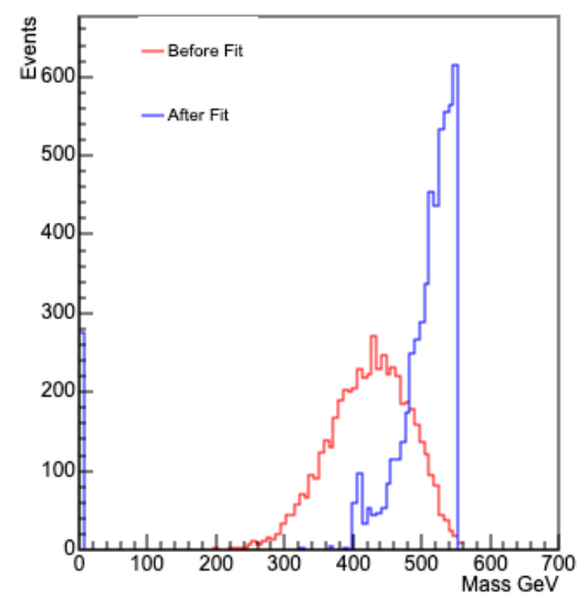
ZHH Mass
