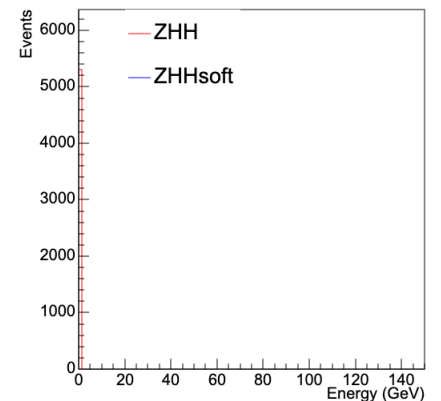
ISR Energy (Prefit)
