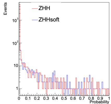
Fit Probability
