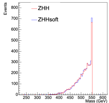
ZHH Mass
