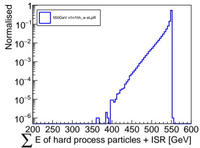
Total energy of initial fermions + ISR
