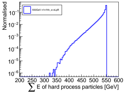
Total energy of initial fermions
