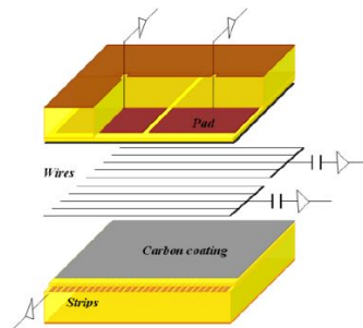
sTGC schematics: 1.8mm wire pitch, 1.4mm wires to cathodes
