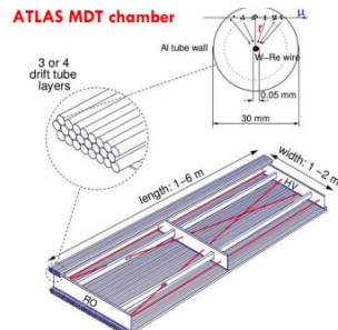
ATLAS MDT chamber
