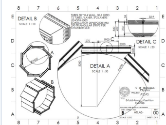
Detector blueprint
