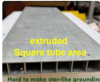
Extruded profile prototype
