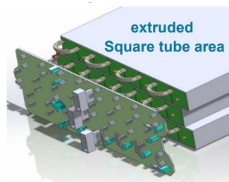
Extruded square tube area
