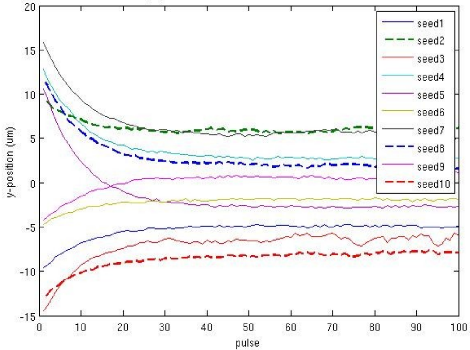
y-position in Fb BPM, FONT=ON, GM=ON
