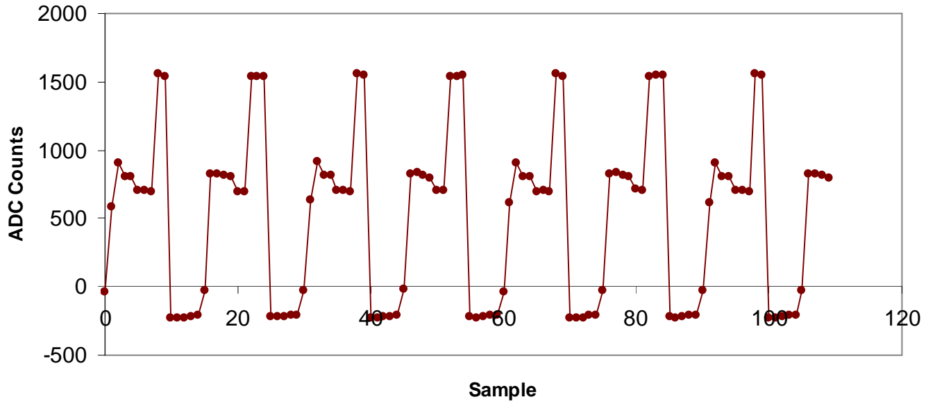
Same arbitrary waveform from FONT4 board using RS232
