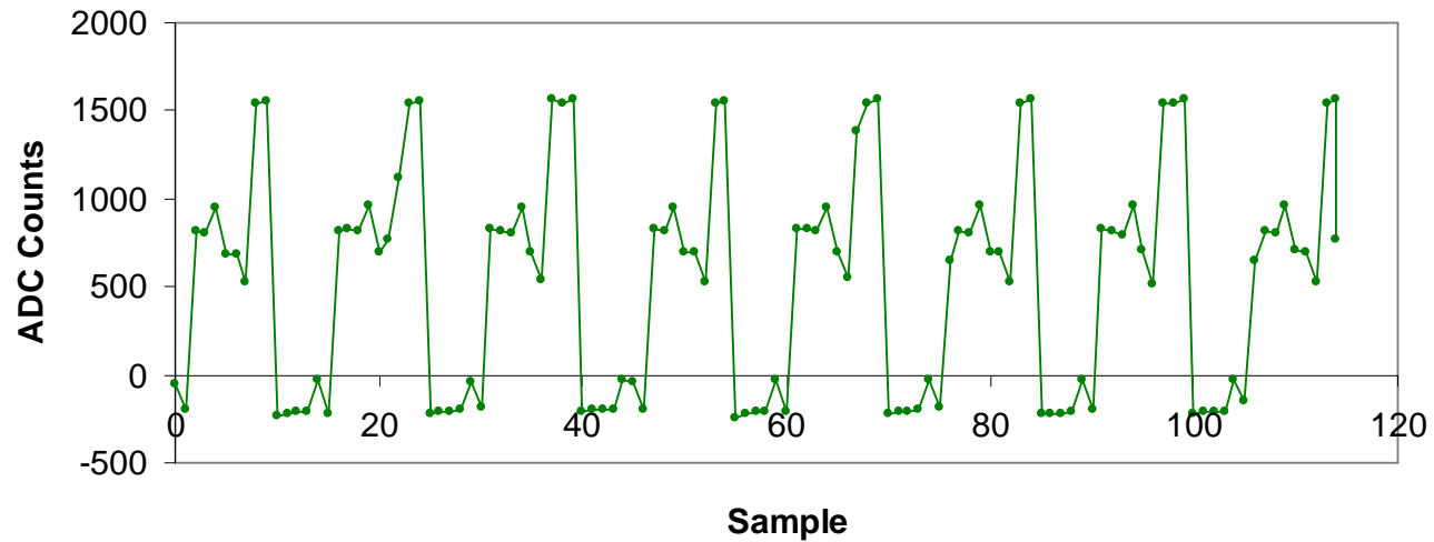
Same arbitrary waveform from FONT4 board using RS232
