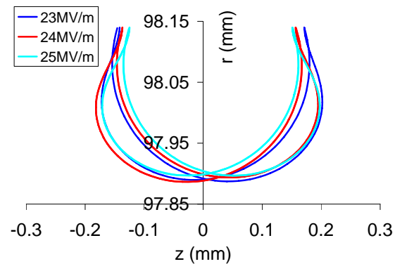
MP trajectories (left) and barriers (right) in regular SRF cells. Soft barrier at around 23MV/m agrees with RF tests.
