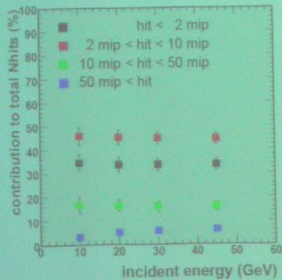
(electron data CERN2006)
