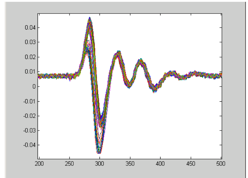
Sum from “processor b” with corrector current of -0.025\text{A}
