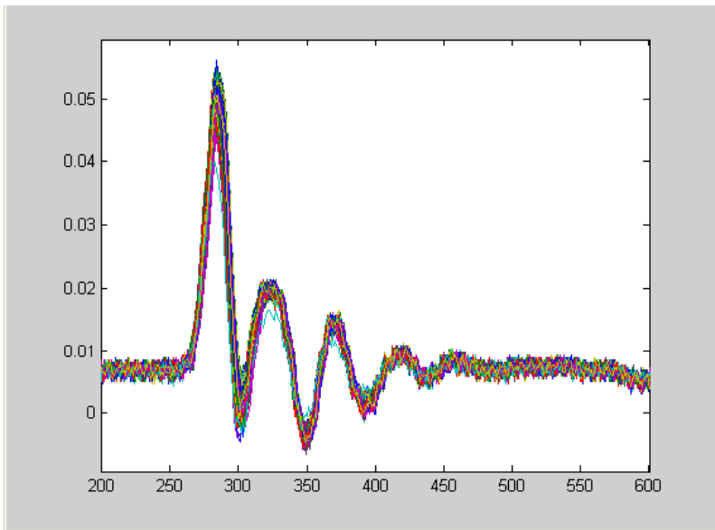
Sum from "processor a" with corrector current of -0.35A
