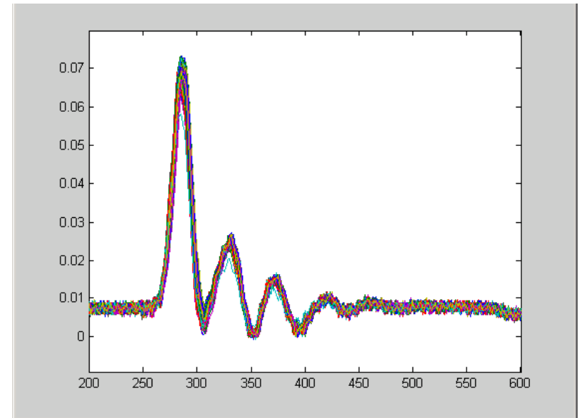
Sum from "processor b" with corrector current of -0.35A
