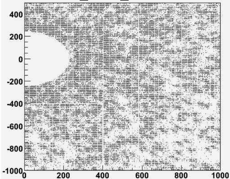
LDC01_06Sc_test
