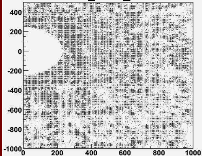
LDCPrime_02Sc_test
