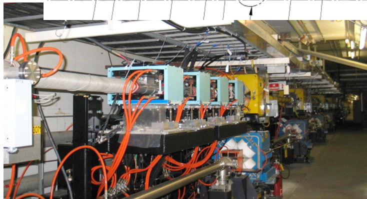
4-dipole chicane in the PEP-II LER
