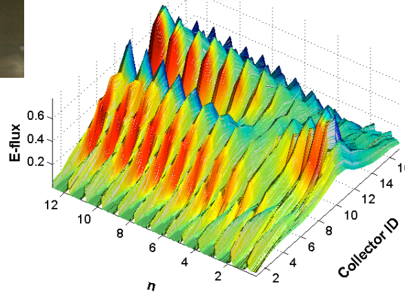
Observed new resonance: Electron current peaks at defined B values ( n )
