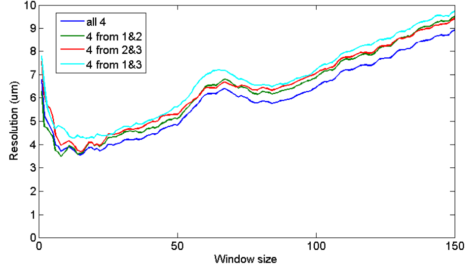
Processor 4 resolution vs window size as predicted from different combinations of processor
