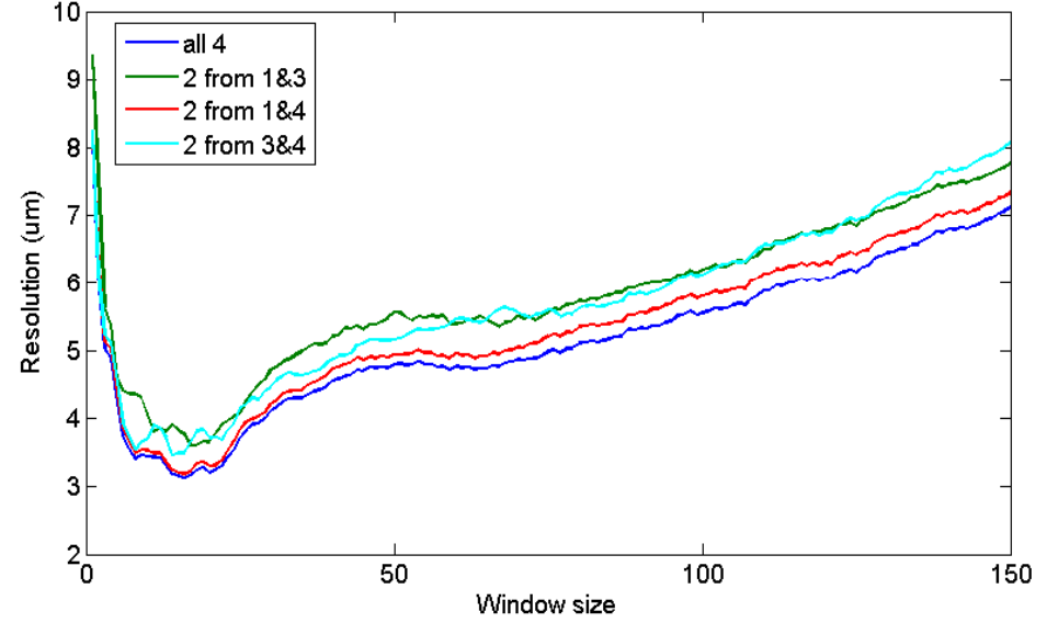
Processor 2 resolution vs window size as predicted from different combinations of processor
