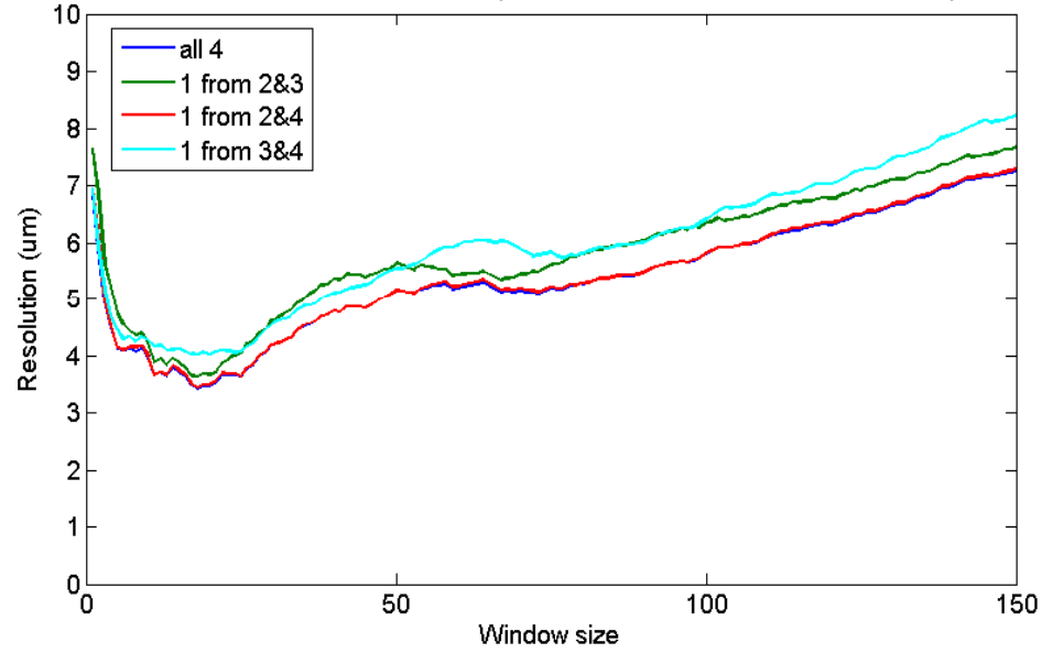
Processor 1 resolution vs window size as predicted from different combinations of processor
