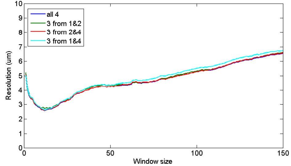
Processor 3 resolution vs window size as predicted from different combinations of processor
