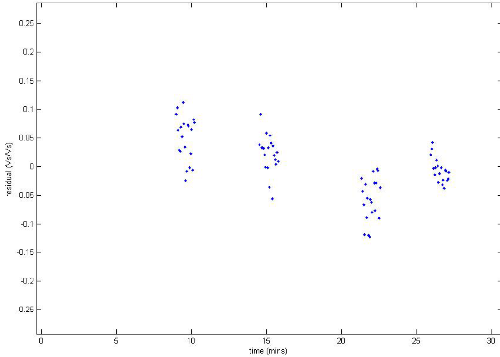
residual vs. time, bunch 1
