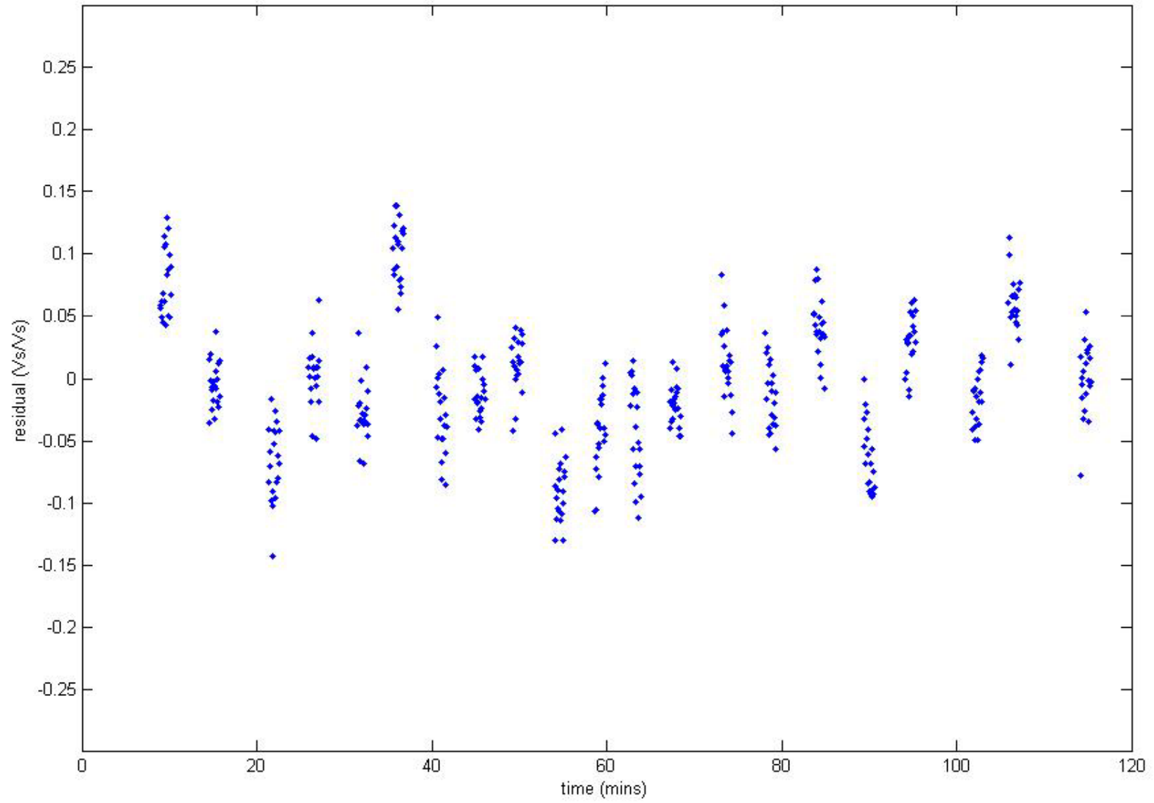
residual vs. time, bunch 3
