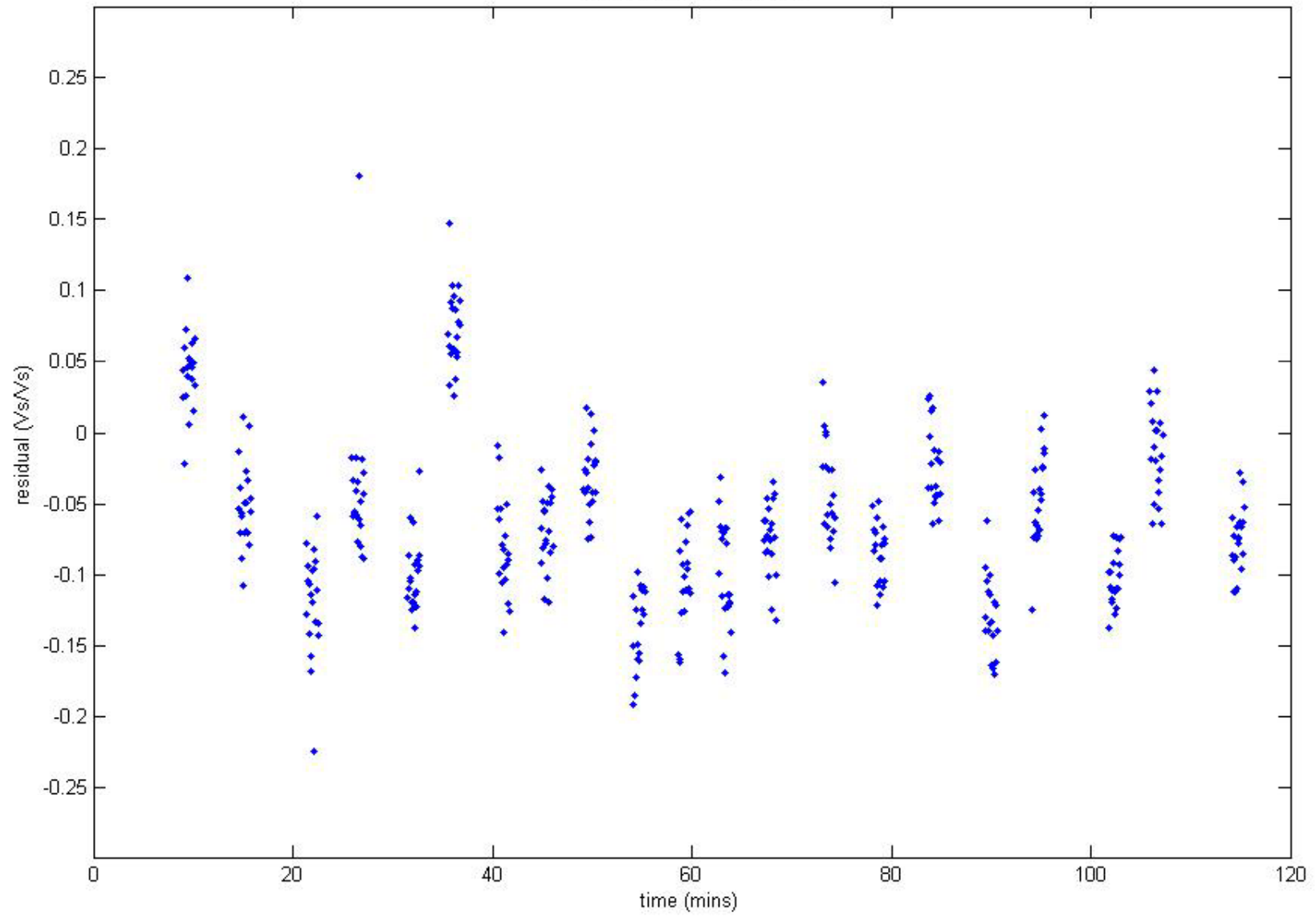
residual vs. time, bunch 2
