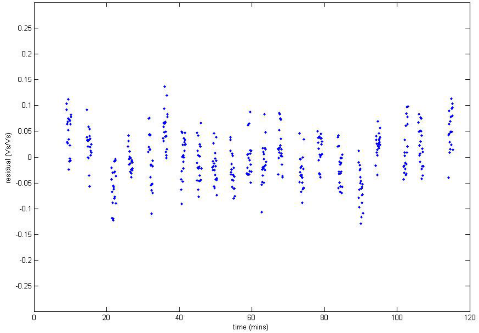
residual vs. time, bunch 1
