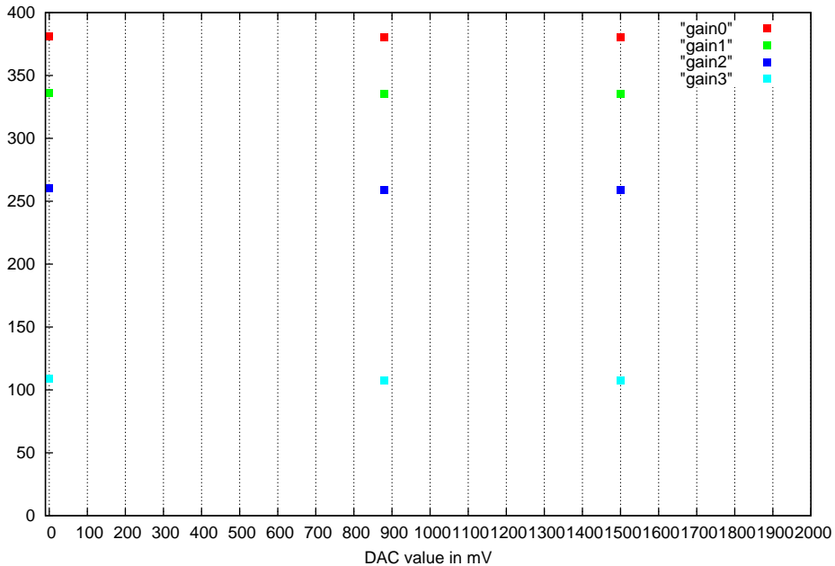
VREF=1200mV, Shaper=0 (80ns), noshaping
