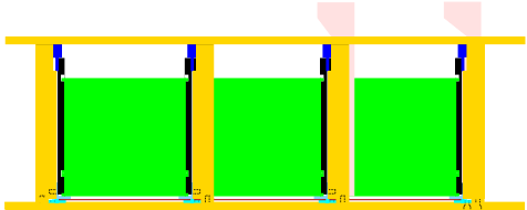
TPC side view (length not to scale)
