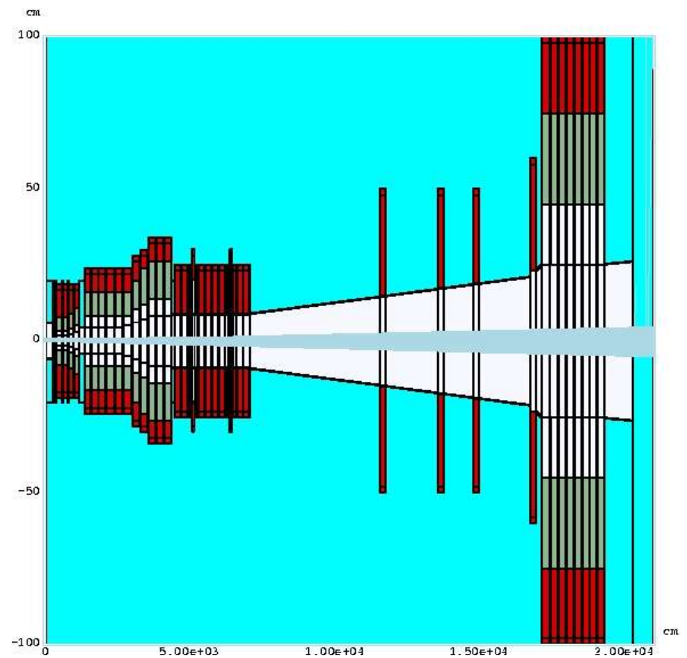
Horizontal view
