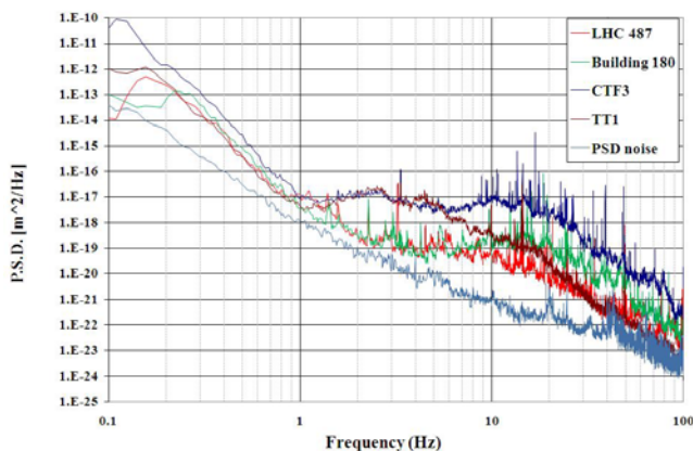
Figure 1: Power Spectral Density of the vertical displacement of the measured sites
