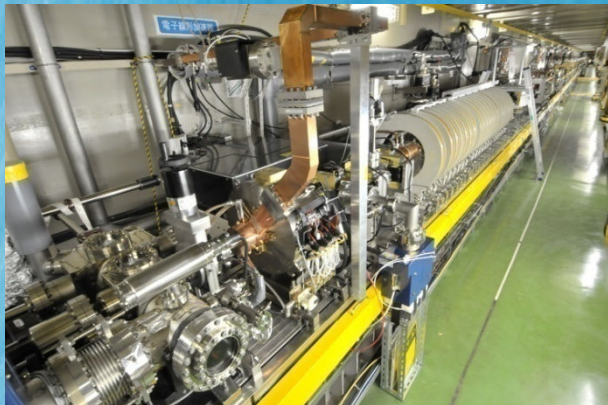
Photo-cathode RF gun (electron source)
