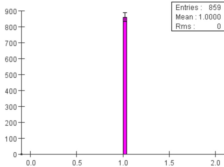
Number of Mip Clusters
