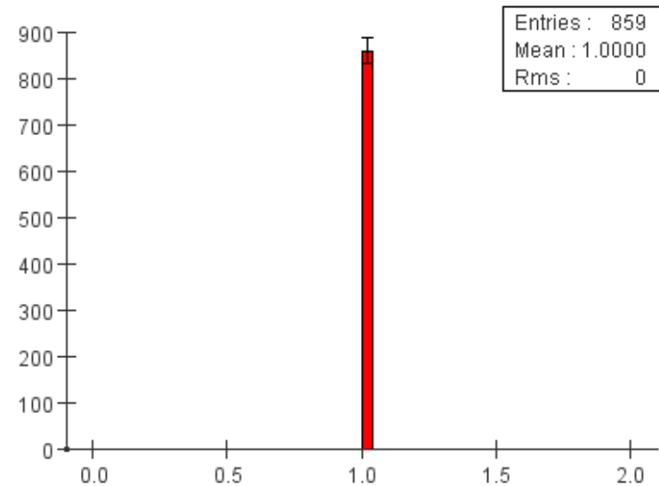
Number of Shower Clusters
