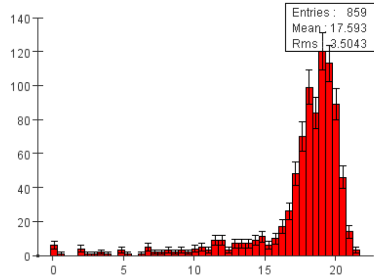
Tr Core Clus E
