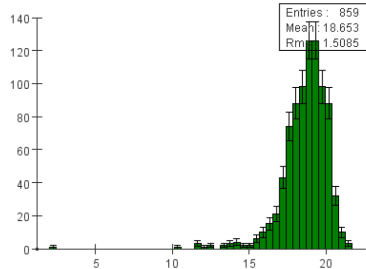
Tr Shower Clus E
