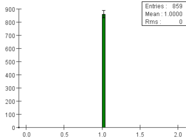
Number of Core Clusters
