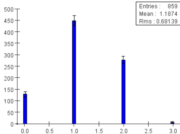
Number of ILSP Clusters
