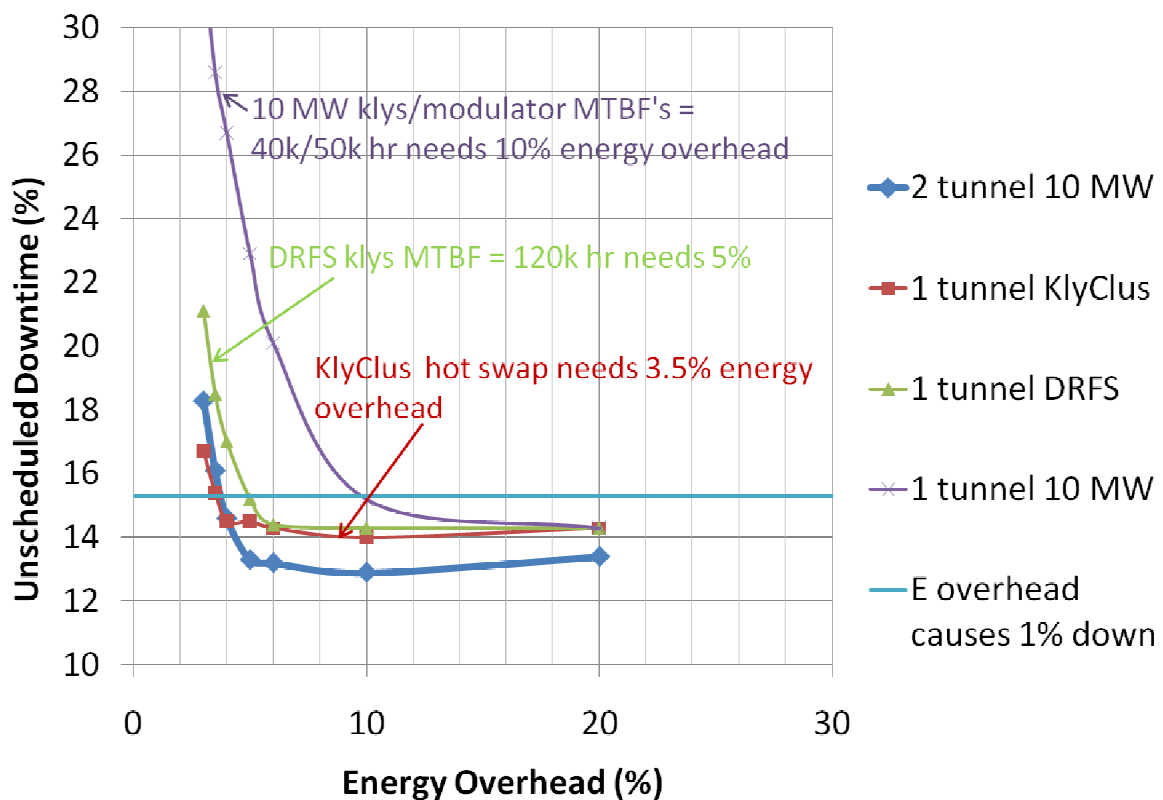
Figure 1. The unscheduled downtime as a function of the main linac energy overhead
