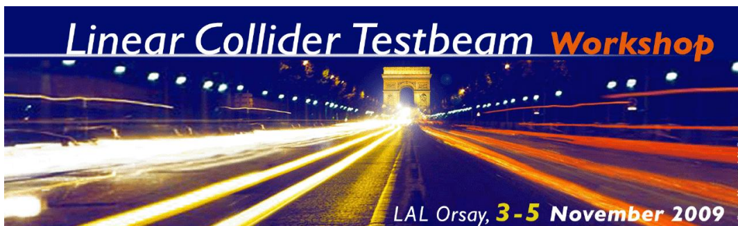
Figure 1: Logo of the Linear Collider Testbeam Workshop 2009.
