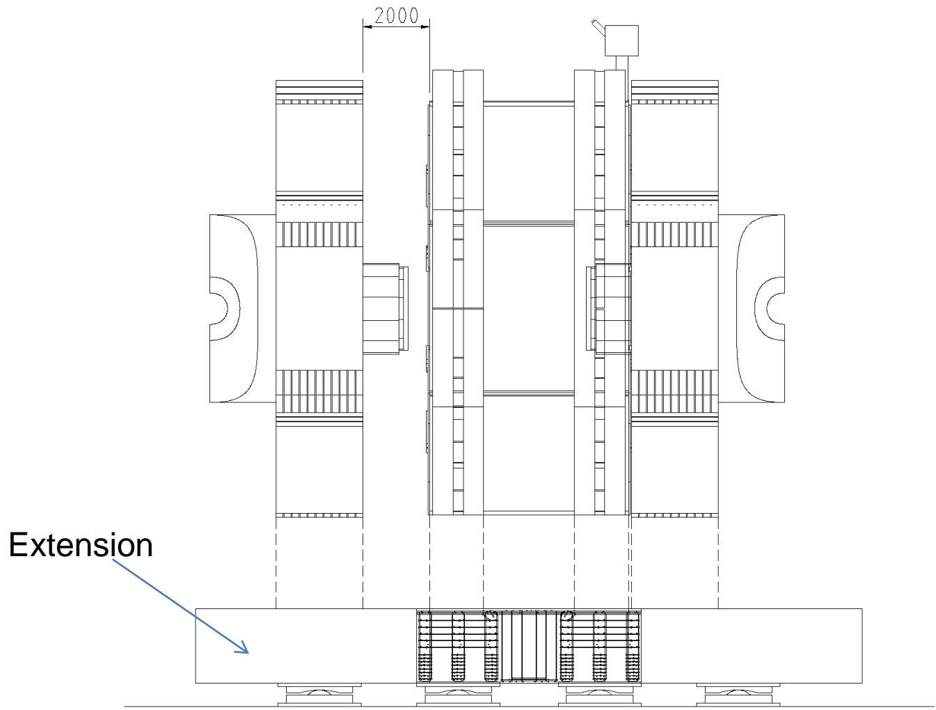
Small Platform (Rigid Cart) + 2 lateral extensions for the opening of the door on the IP
