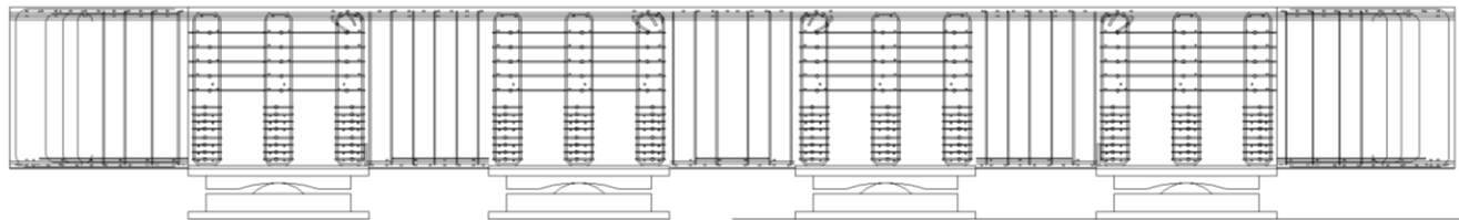
Modification Needed for Push Pull (multi supports with reinforcements)
