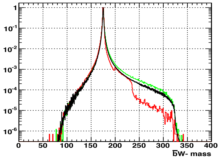
\bar{b}W^- (em+1.0,ep0.0)
