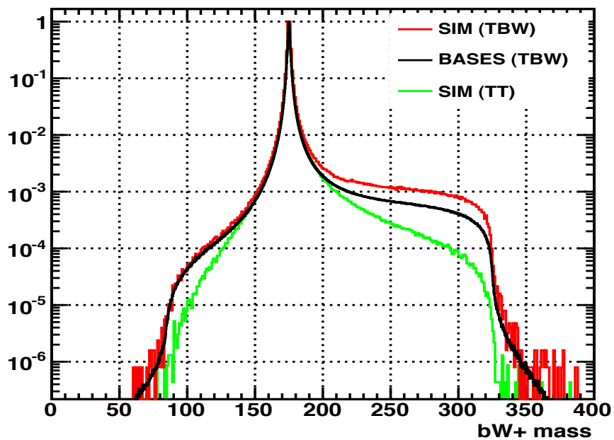
bW+ (em+1.0,ep0.0)
