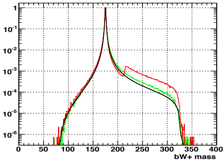
bW+ (em+1.0,ep0.0)
