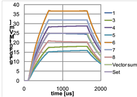
Figure 7: LLRF control to compensate the Lorentz force detuning, and the vector sum stability in S1-Global cavity-string test.
