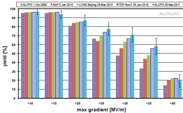
Figure 4: Cavity gradient performance progress with production yield for the second pass as of March 2011.
