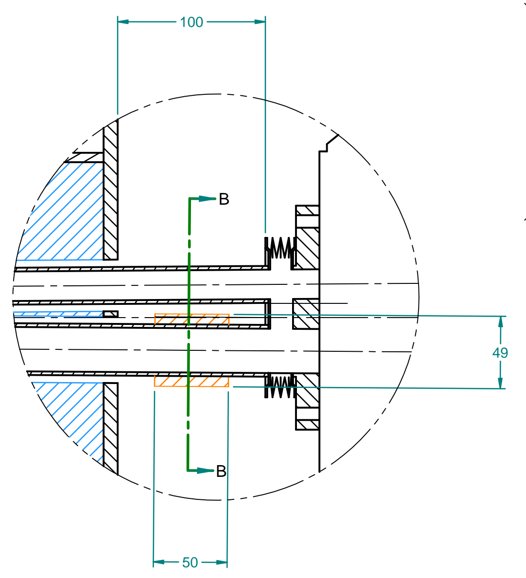
DETAIL A SCALE 4:1
