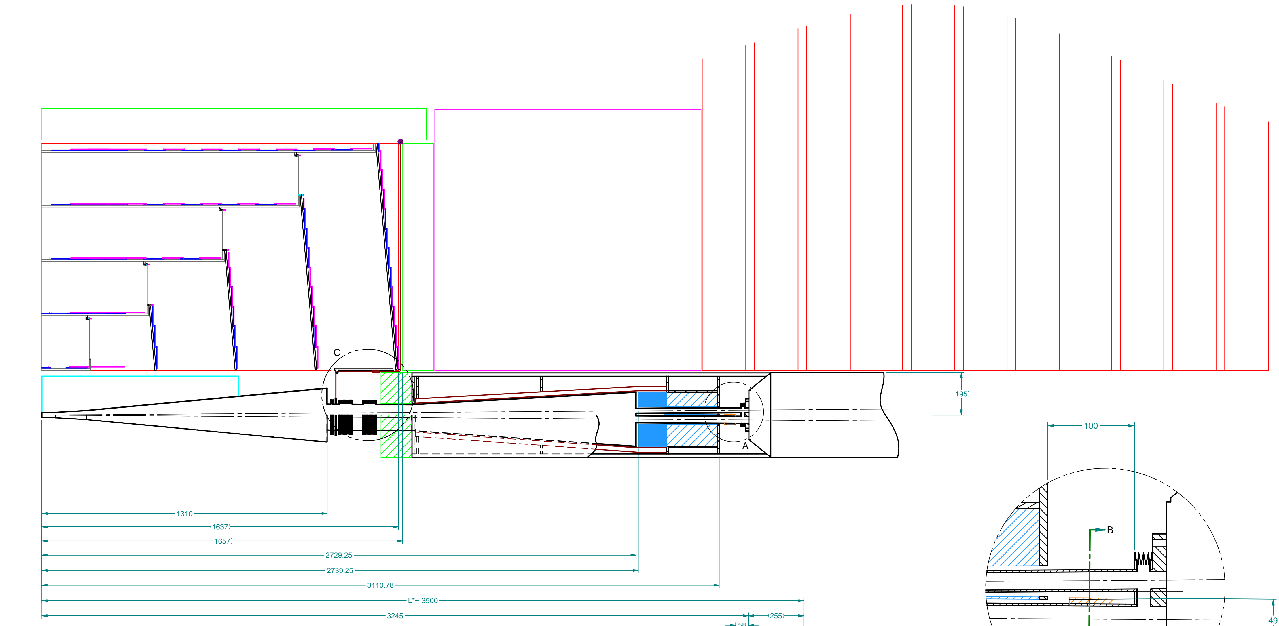
SECTION B-B SCALE 4:1
