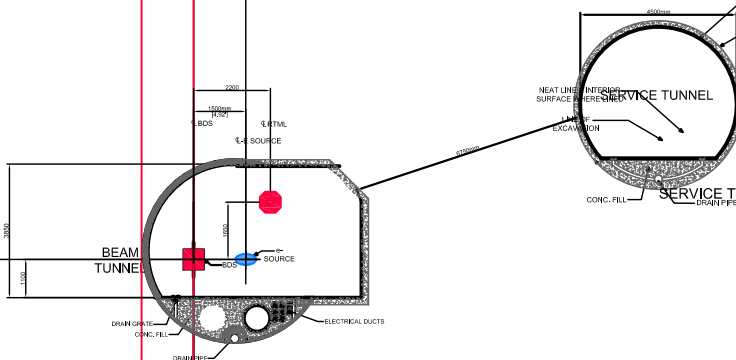
e+ MAIN LINAC : AFTER TRANSITION OF e- SOURCE TO CEILING (D)
