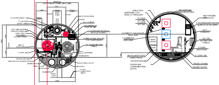
5.0M Q2 TUNNEL SECTION @ e+ MAIN LINAC (A) DAMPING RING SHOWN FOR REFERENCE ONLY
