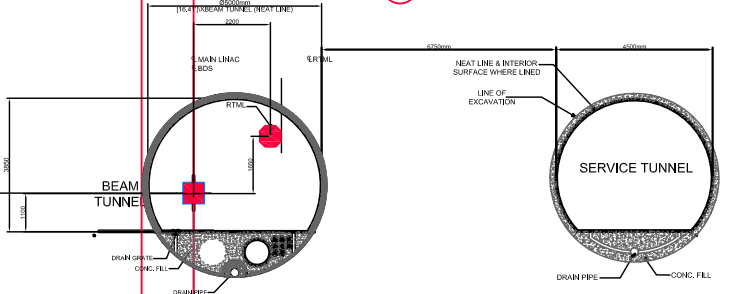
e+ MAIN LINAC : SECTION FROM MAIN LINAC TO e- GUN (B)
