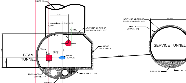
e+ MAIN LINAC : SECTION FROM e- GUN TO 100M PAST 5 GeV LINAC (C)
