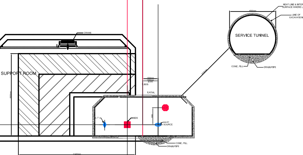
e+ MAIN LINAC : SECTION @ BDS NEAR DETECTOR HALL (E)
