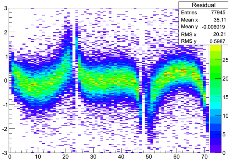
RUN3127 B=0T Phi=15°
