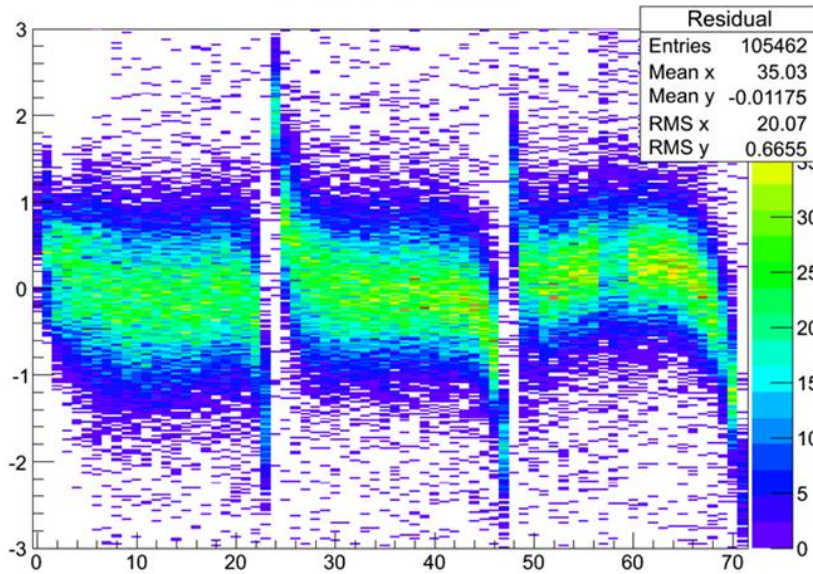
RUN3124 B=0T Phi=20°
