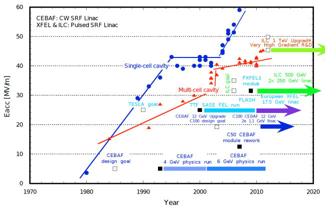
Fig. 14: SCRF cavity field gradient progress and future prospect.
