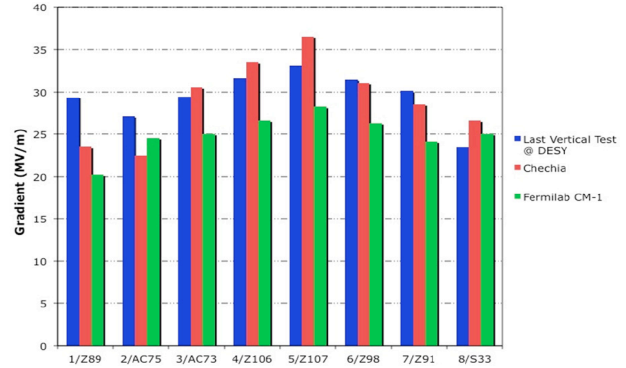
Fig. 9: Field gradient achieved in the CM1 cryomodule developed at Fermilab10].
