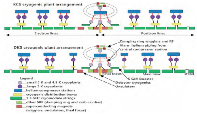
Fig. 12. Cryogenics facility layout for the ILC cryogenics.
