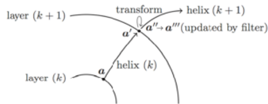
Figure 1 : The updated track propagation procedure.
