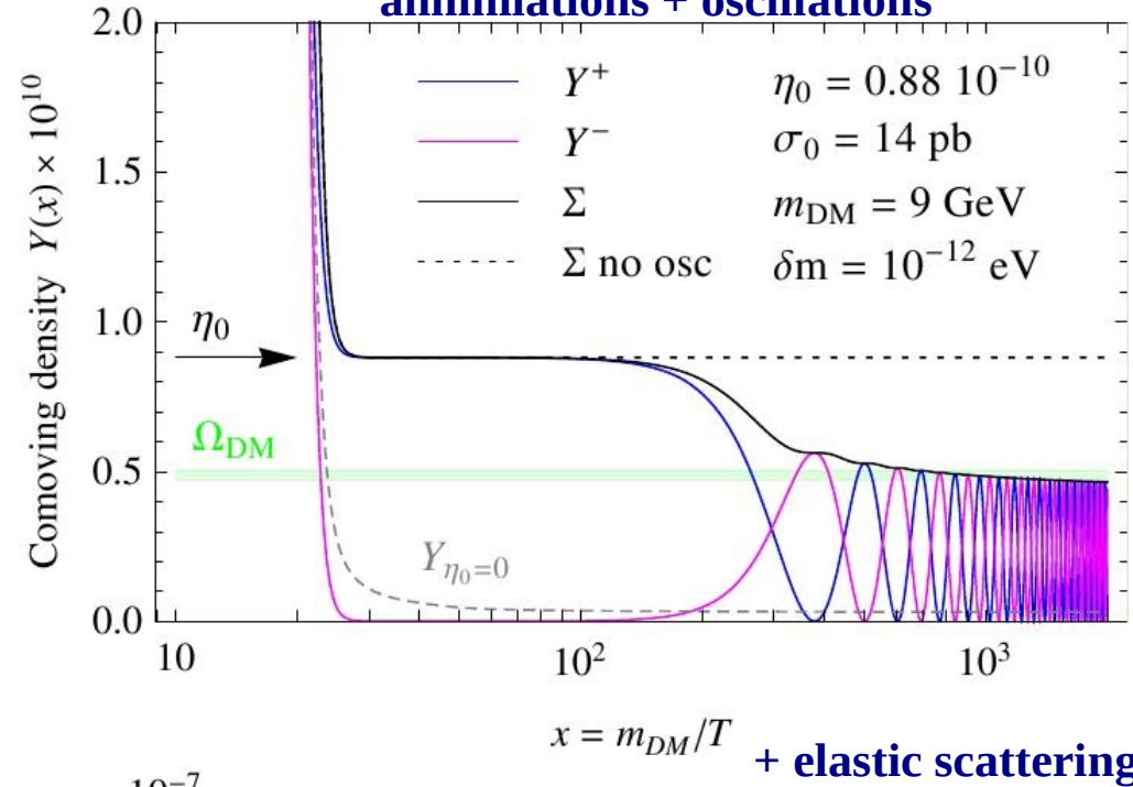
annihilations + oscillations
