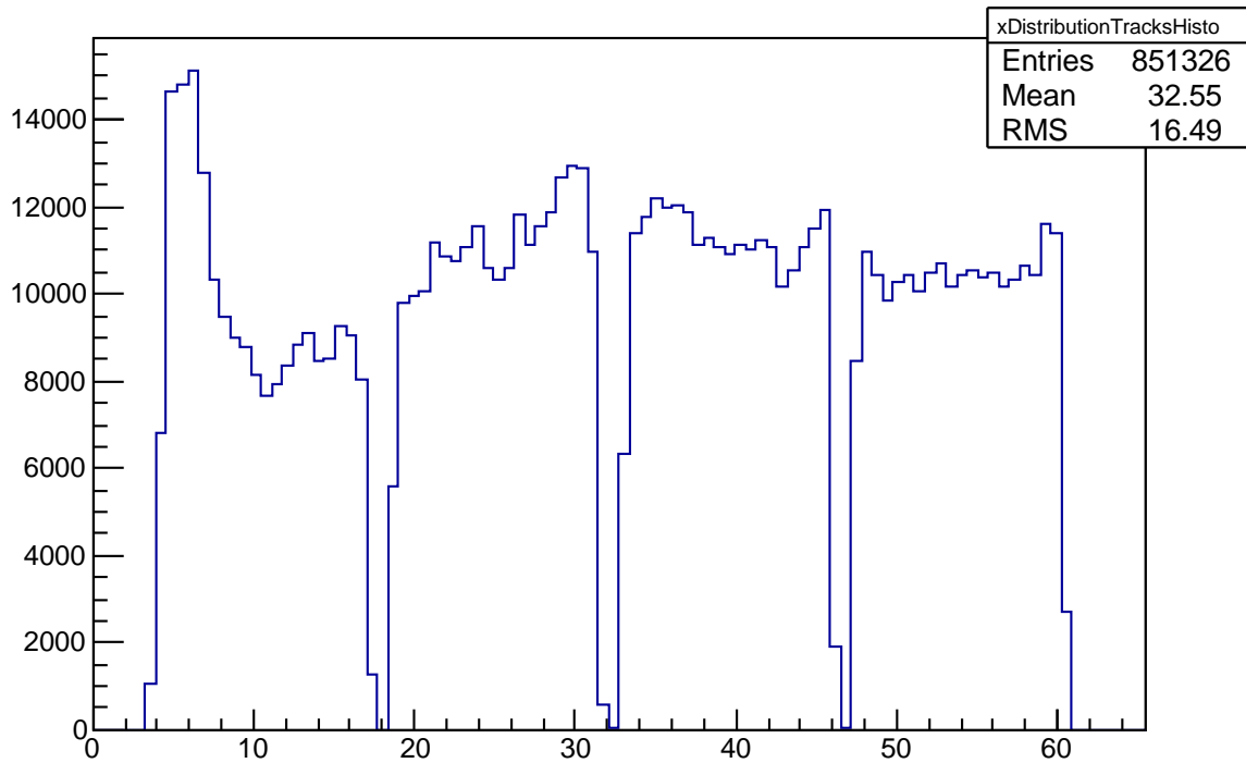
xDistributionTracksHisto
