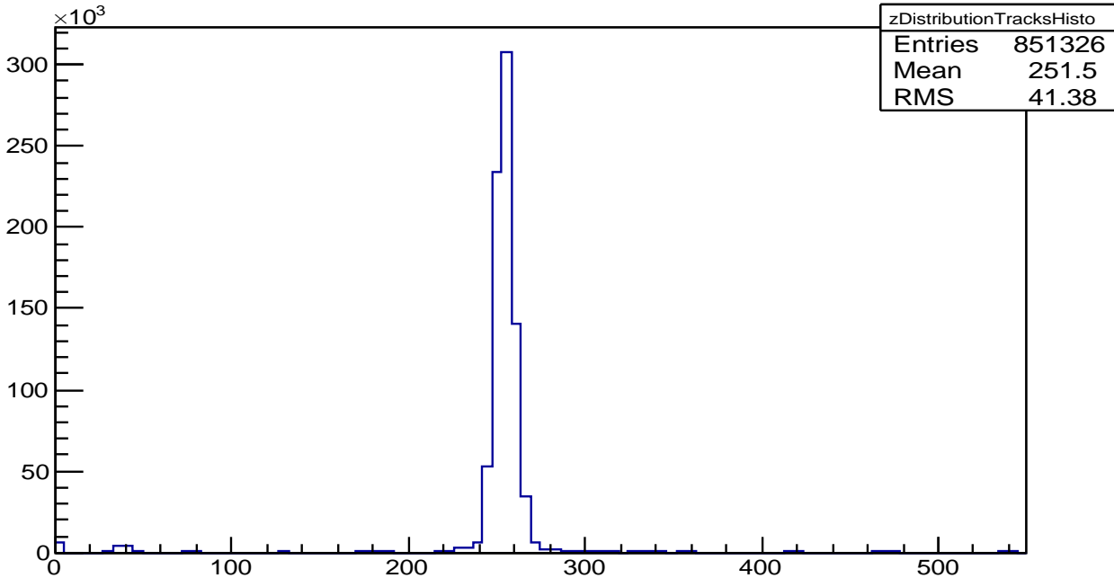
zDistributionTracksHisto
