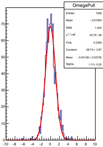
Omega pull
