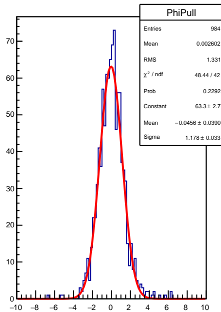
Phi pull
