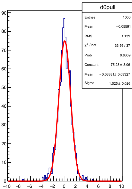
d0 pull
