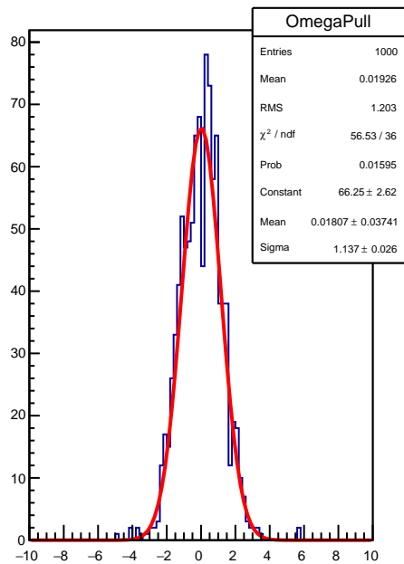
Omega pull
