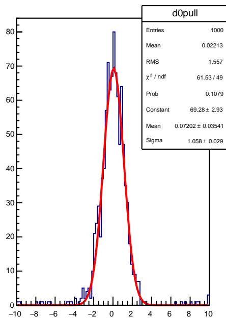
d0 pull
