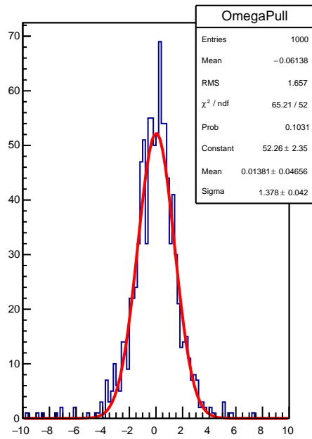
Omega pull
