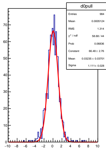
d0 pull
