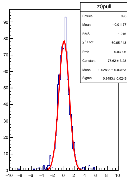
z0
