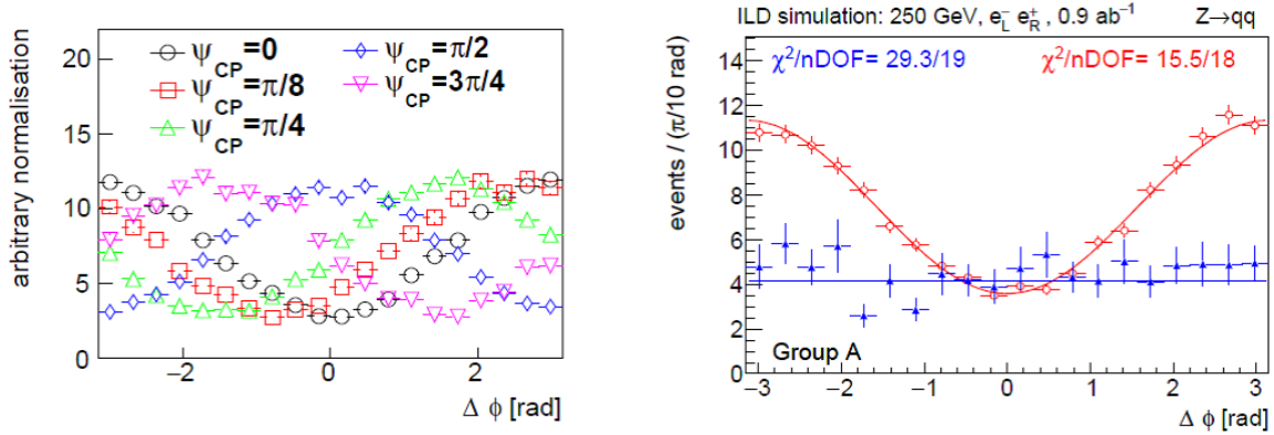
Figure 3 – Left: distribution of the CP-sensitive correlation angle for different CP mixing cases at the generator-level. Right: reconstructed angular distribution in the case of the SM, for a sub-sample of selected events; signal is shown in red and background is blue.
