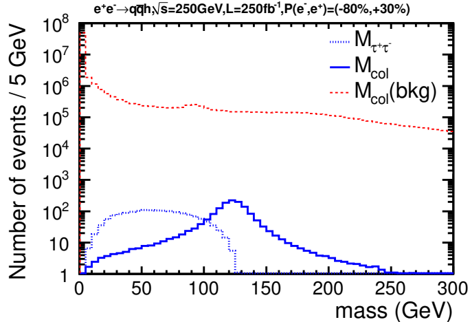
Figure 1 – Reconstructed \tau -pair mass in H \rightarrow \tau^+\tau^- analysis 3 . Dotted blue is the invariant mass of \tau -pair only using visible \tau decay products in the signal process, solid blue (dotted red) is the invariant mass of \tau -pair with using collinear approximation in the signal (background) process, respectively.
