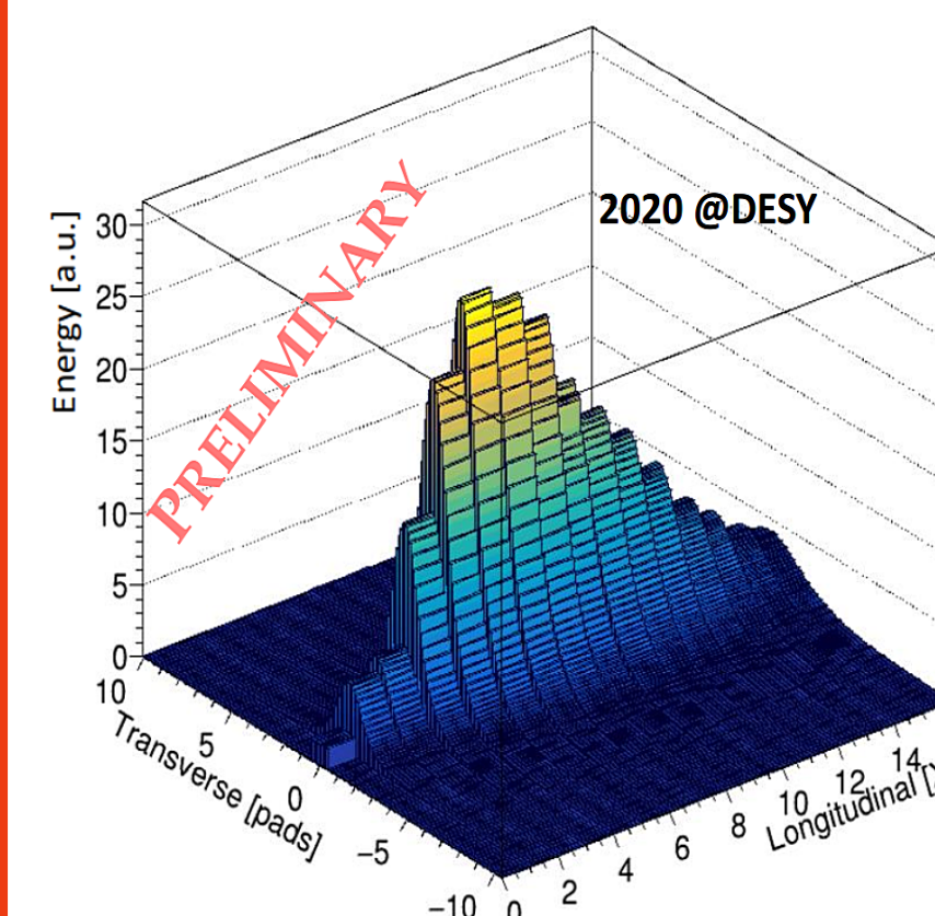
A lego plot of the transverse profile for each layer from the test-beam data
