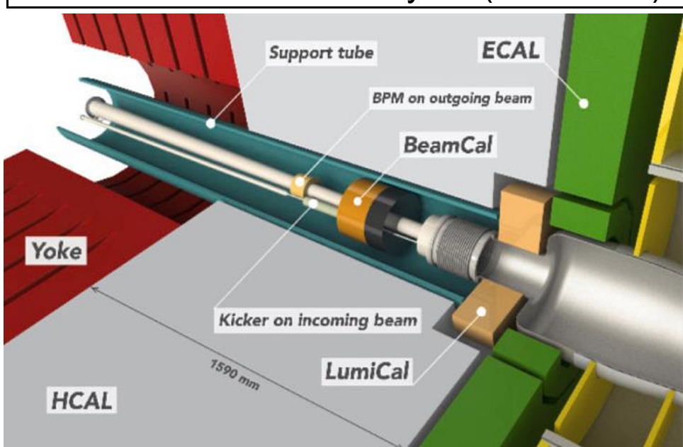
CLICdet forward region
