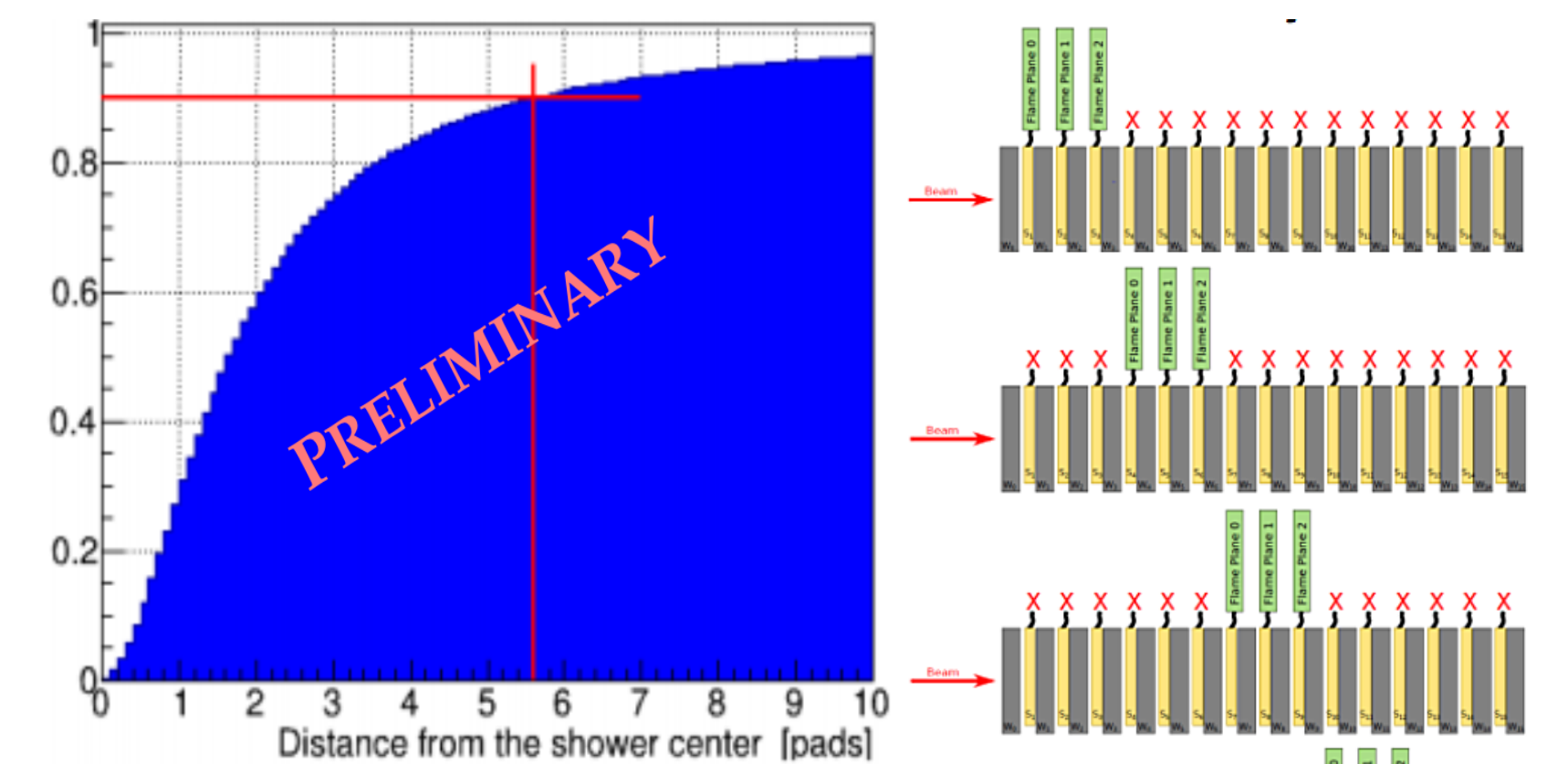
The integral on F_E(r) , that was extracted from the fit, as a function of the distance in units of pads (1.8mm) for 5 GeV e^- beam
