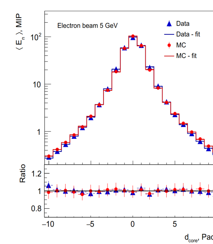
The transverse shower profile \langle E_T \rangle , as a function of d_{core} in units of pads.
