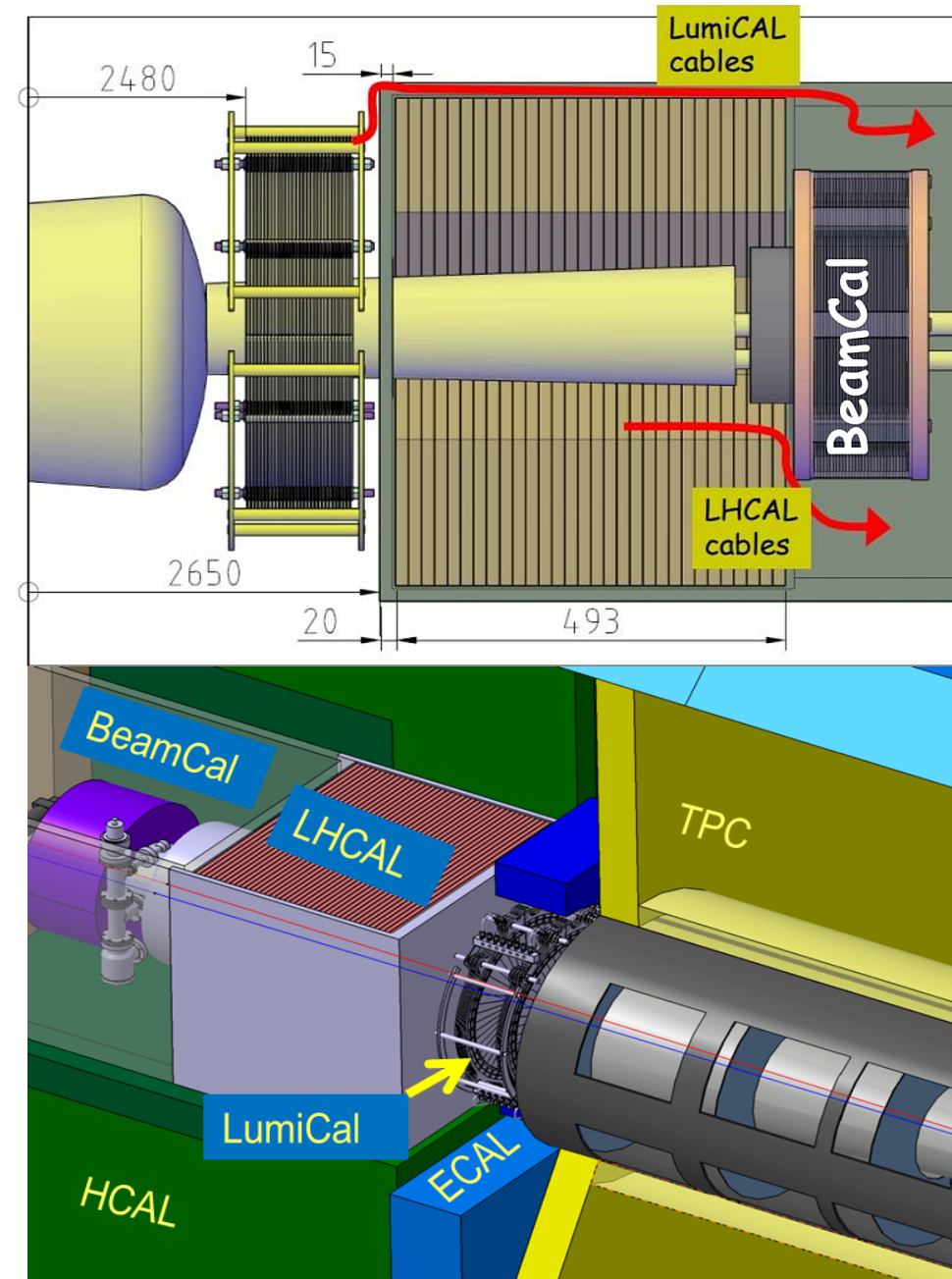
ILD forward region
