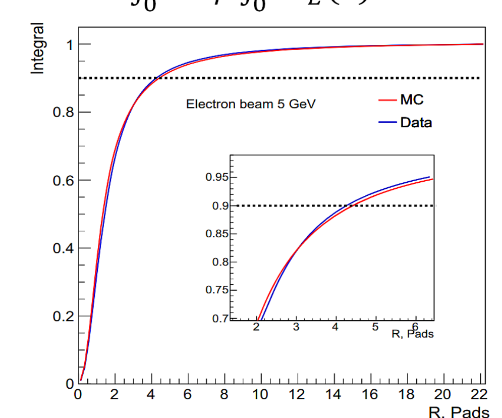
The integral on F_E(r) , extracted from the fit, as a function of the radius, R , in units of pads (1.8mm)
