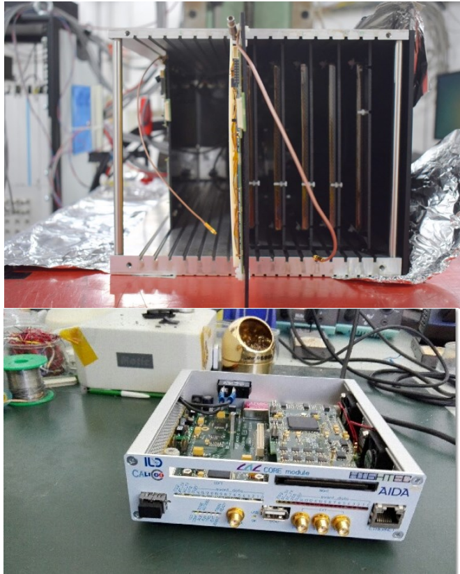
ECAL testbeam campaign at DESY
