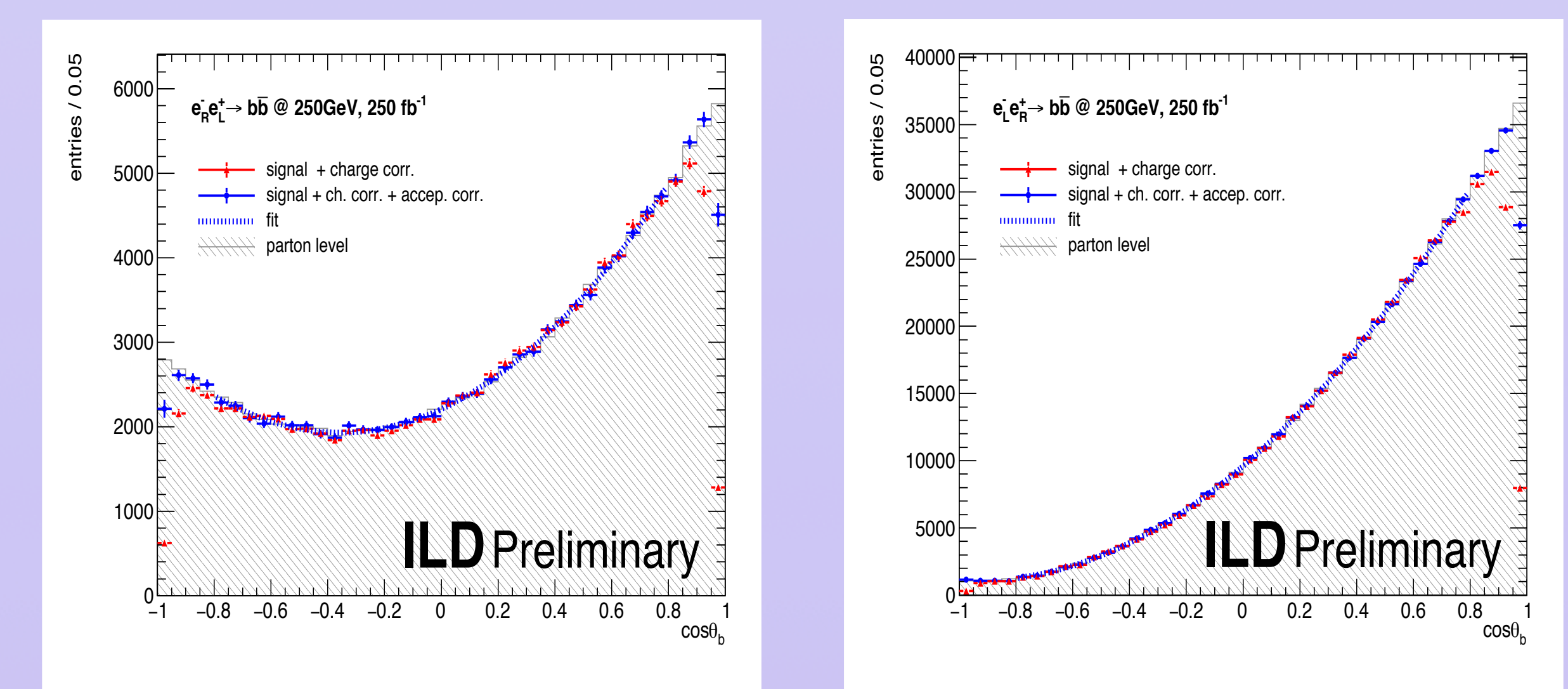
Figure 8 Polar angle distributions for left-handed (left) and right-handed (right) bottom quarks.
