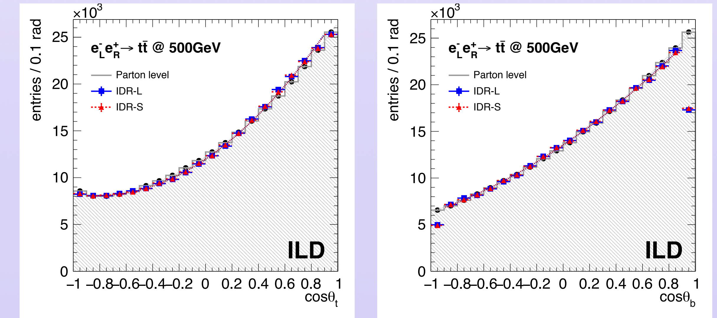
Figure 7 Polar angle distributions for left-handed top quarks (left) and its decay product, bottom quarks (right) is presented. Both of which are scaled with its efficiencies.
