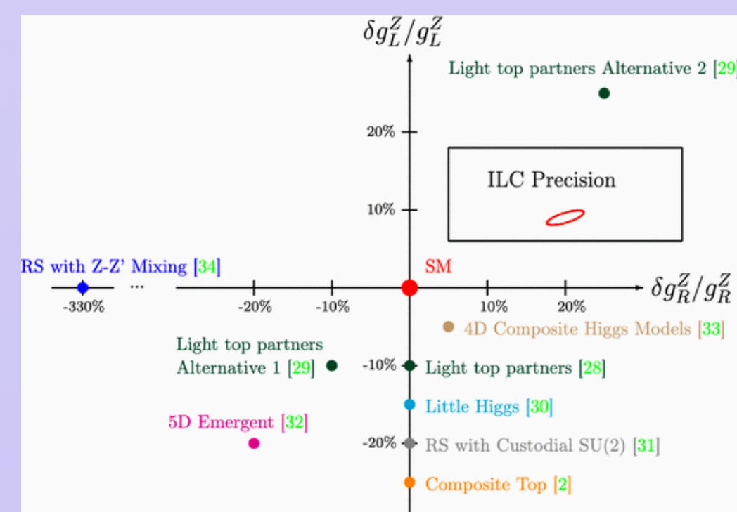
Figure 2 Deviation of ttZ coupling for right and left handed top quark. [1]
