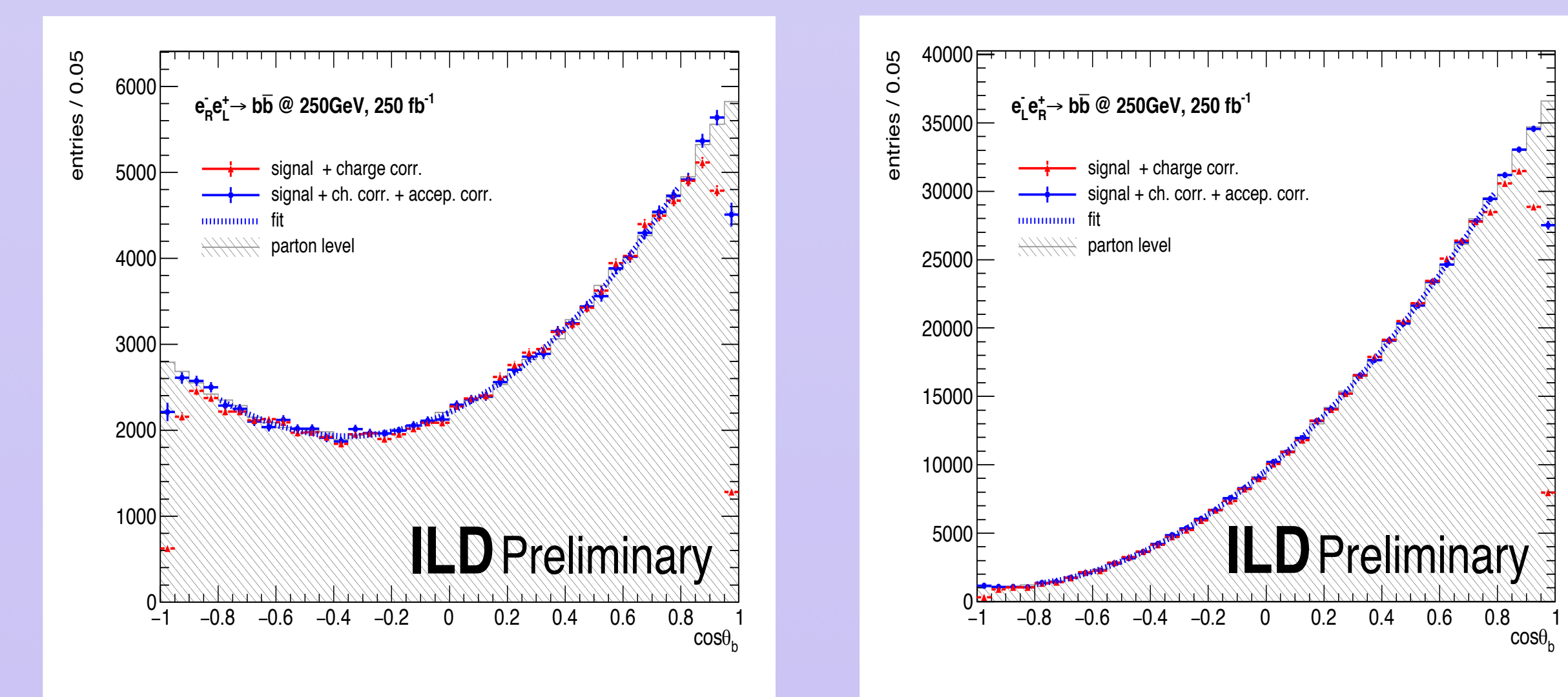
Figure 8 Polar angle distributions for left-handed bottom quarks
