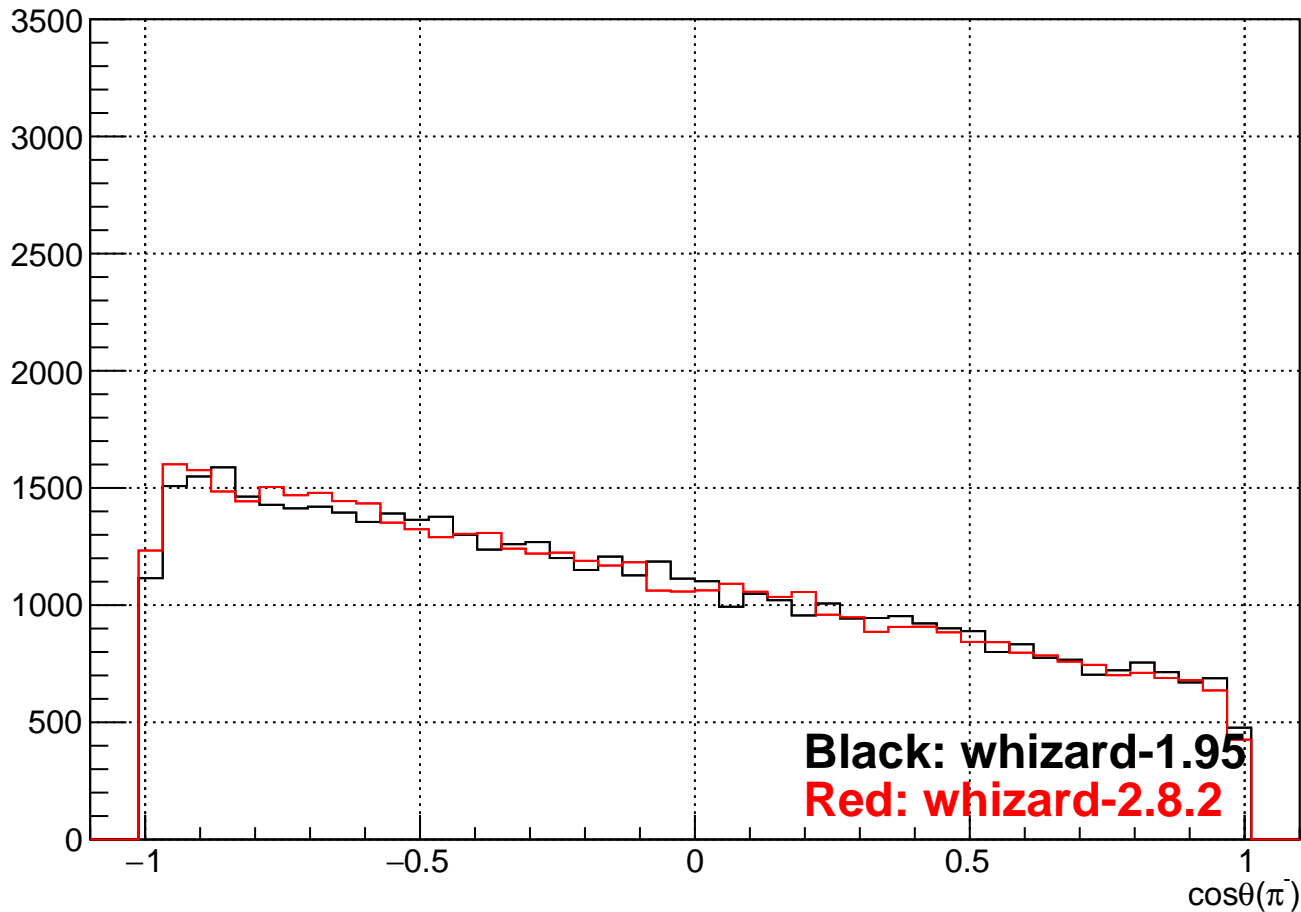
\cos\theta(\pi) in \tau^+\tau^- system: \tau^+\tau^- ISR on, BSoft, \tau\rightarrow\pi\nu @ 250 GeV
