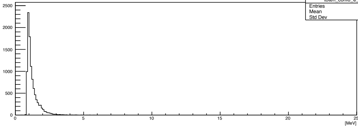
Total Energy conf0_e_3GeV
