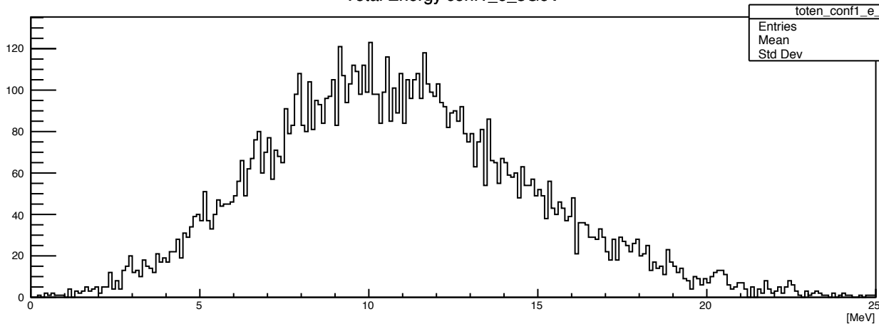
Total Energy conf1_e_3GeV
