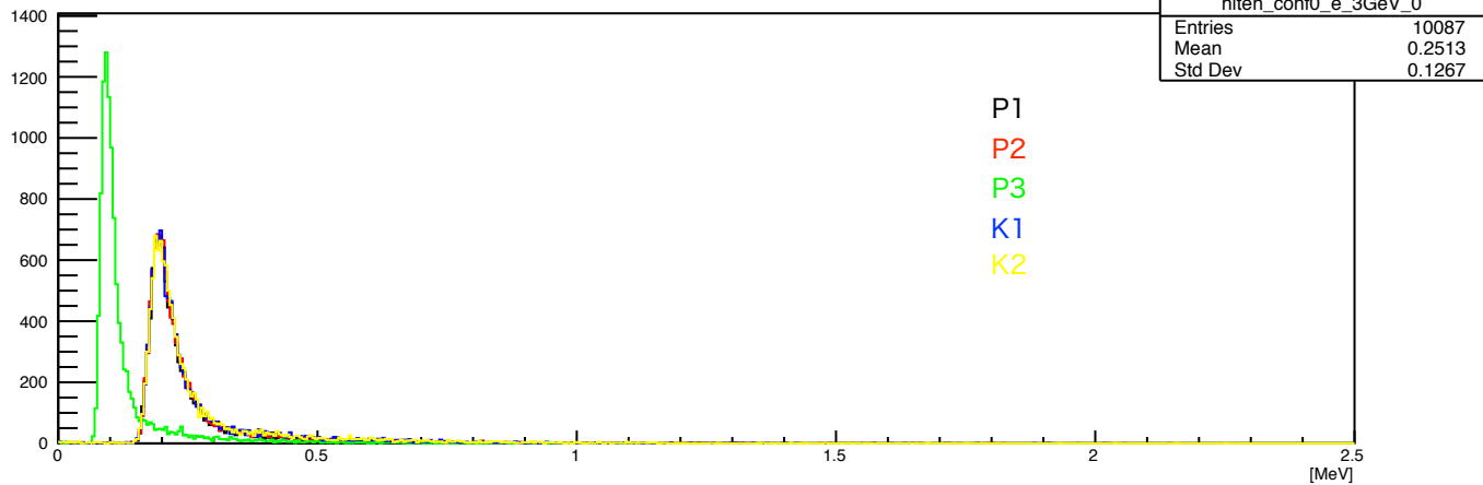
Hit Energy conf0_e_3GeV
