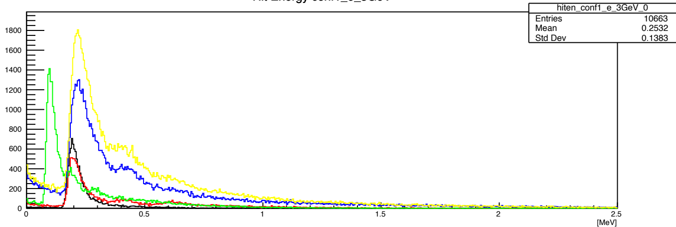
Hit Energy conf1_e_3GeV
