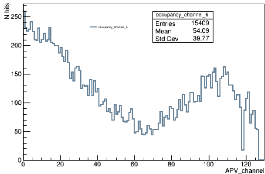
occupancy_channel_6
