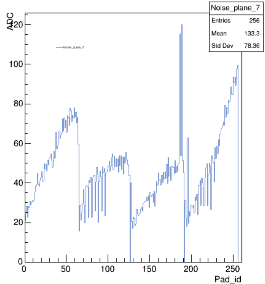
Noise_plane_7
