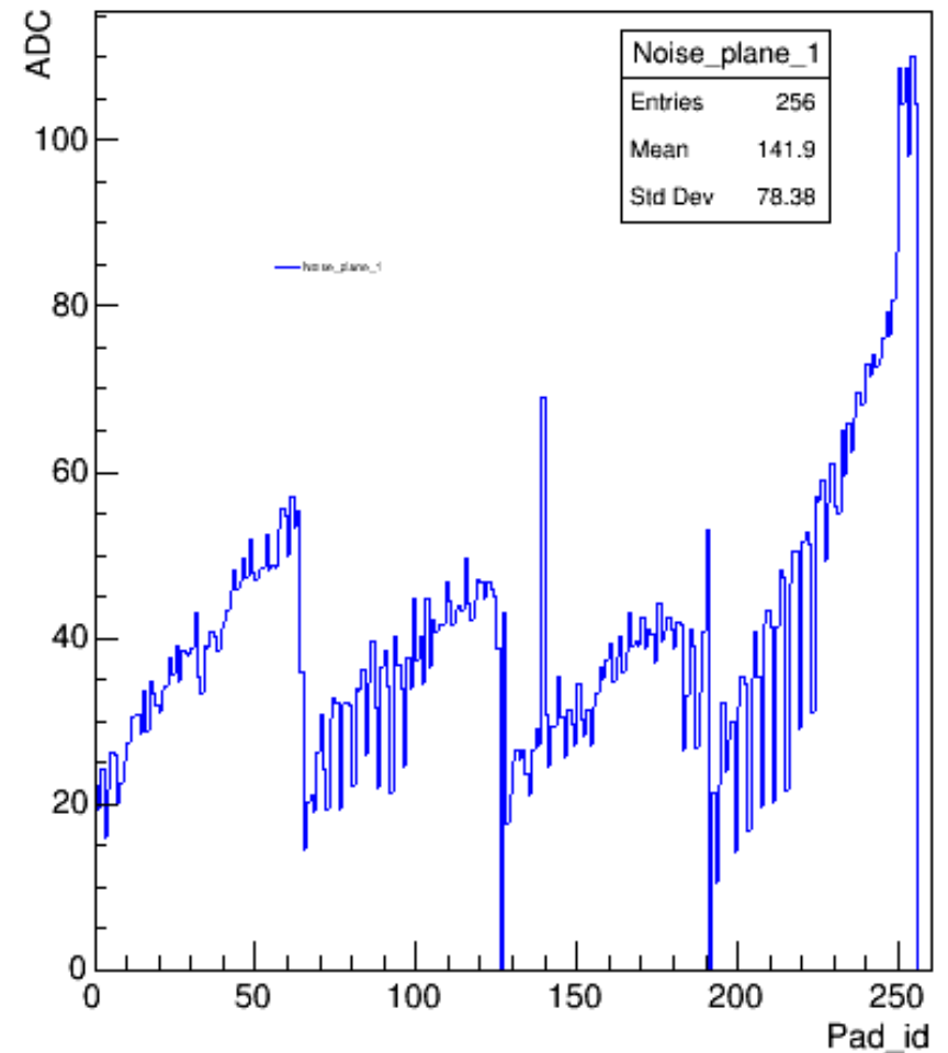
Noise_plane_1
