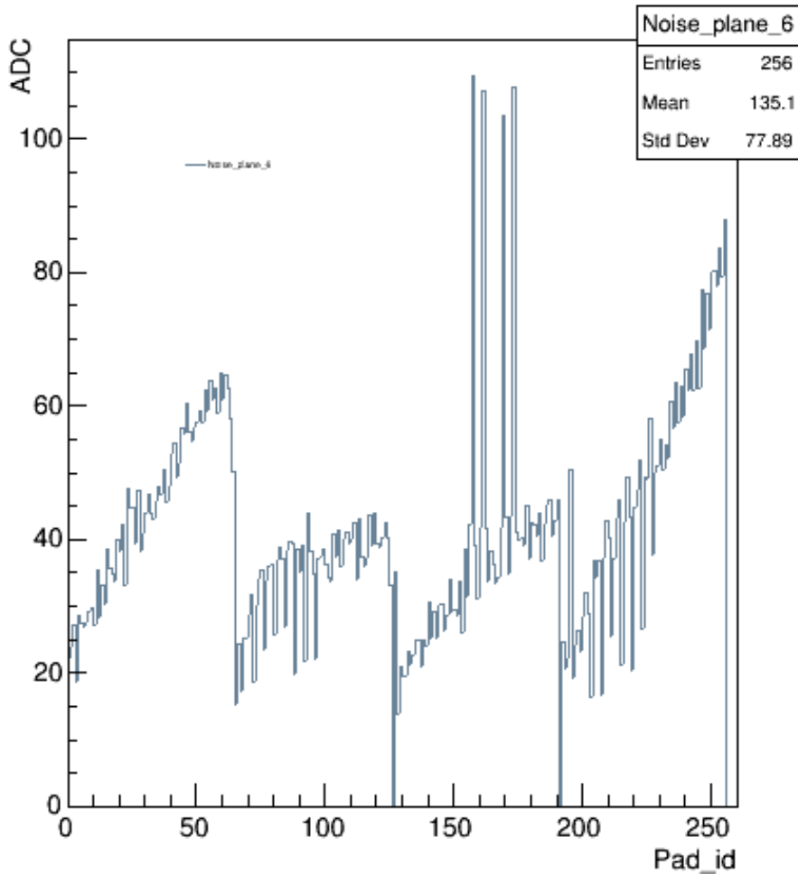
Noise_plane_6
