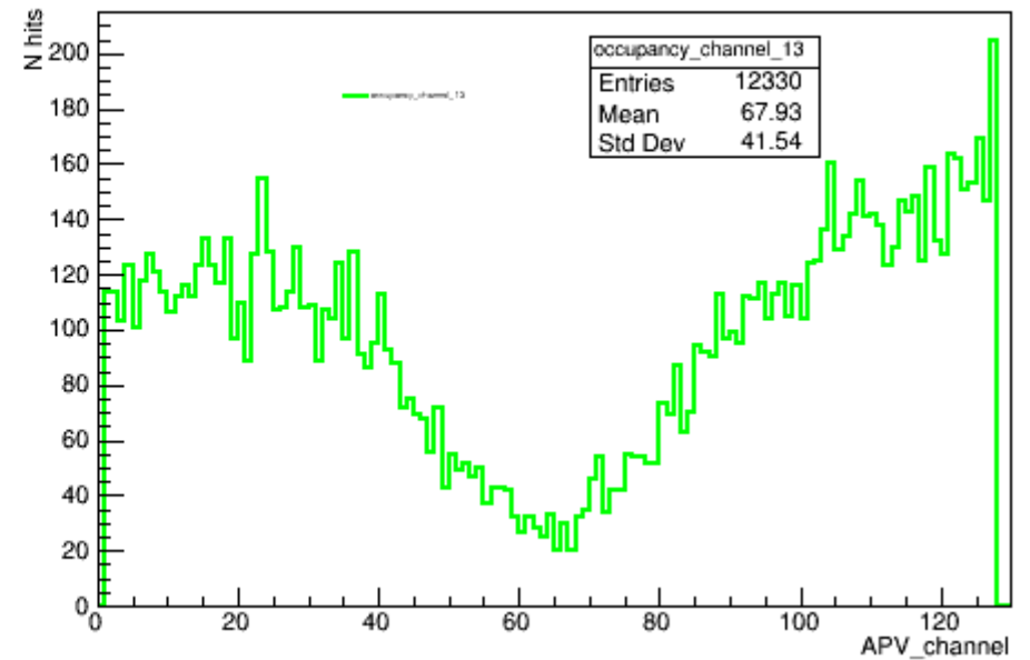
occupancy_channel_13
