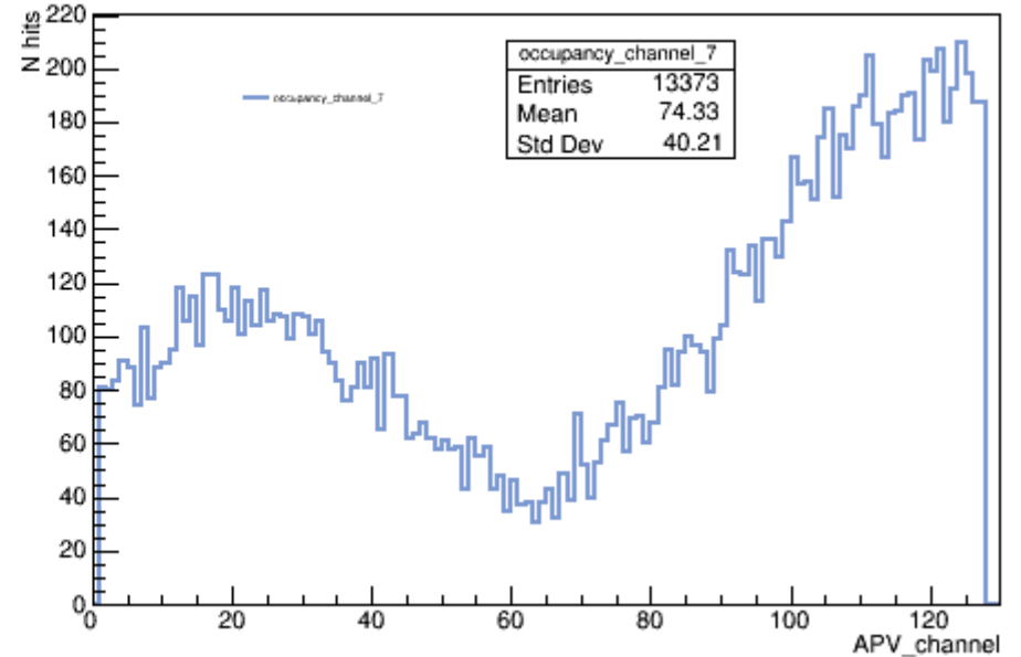
occupancy_channel_7
