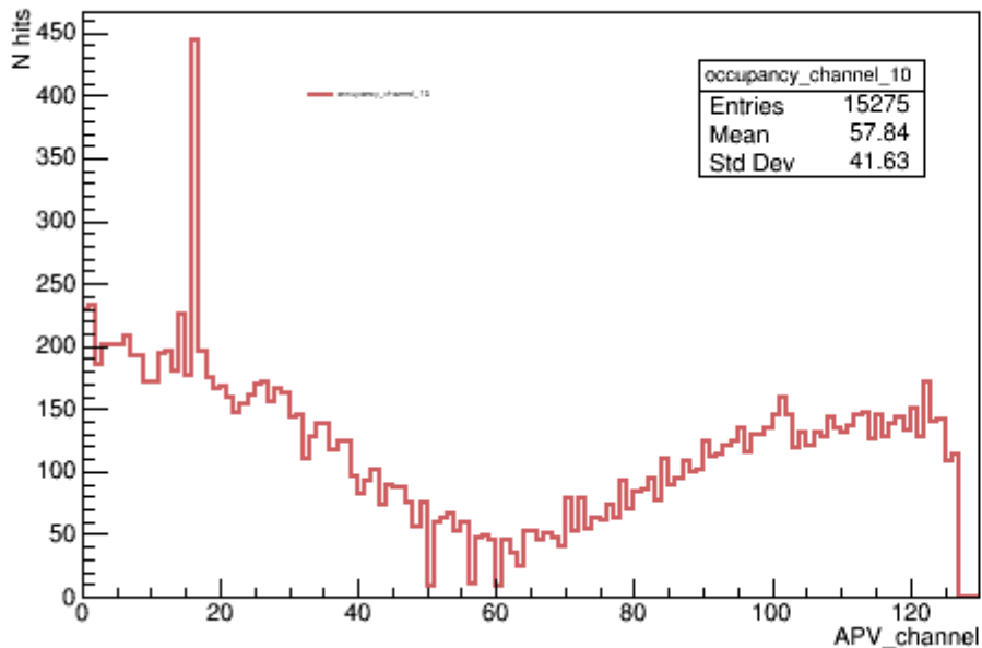
occupancy_channel_10
