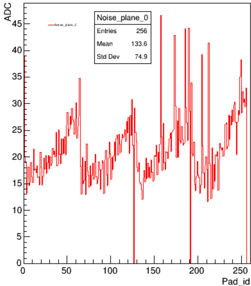
Noise_plane_0
