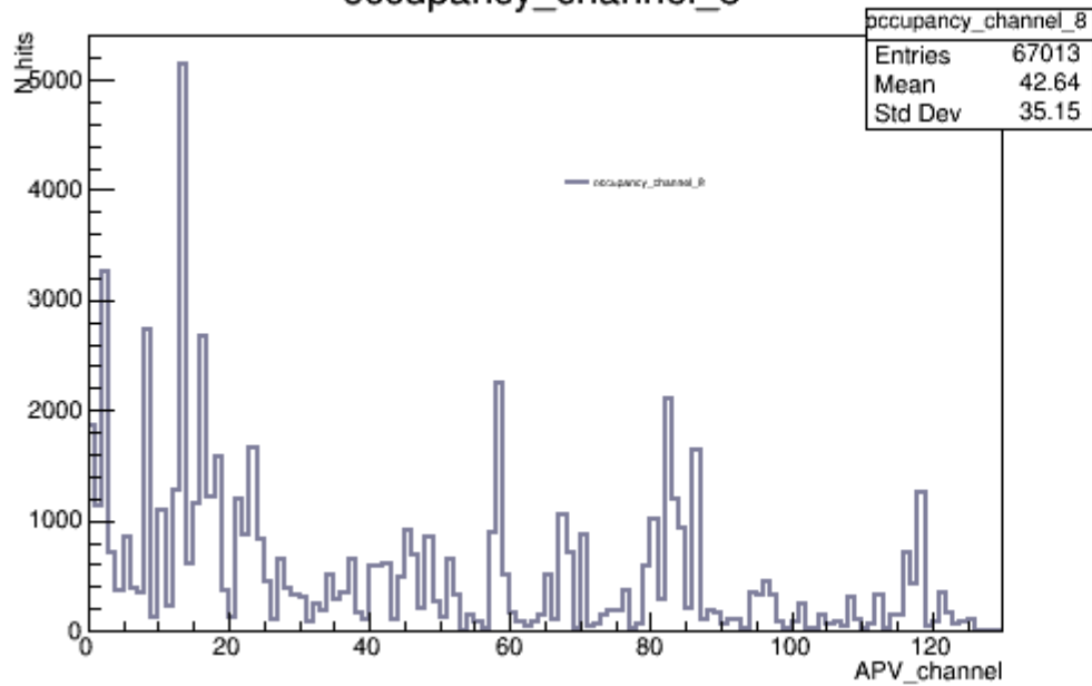
occupancy_channel_8
