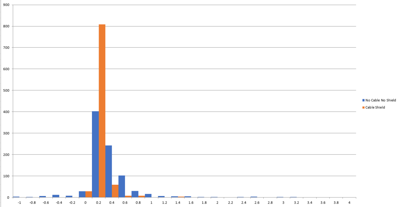
Crosstalk (%) Distribution Fine
