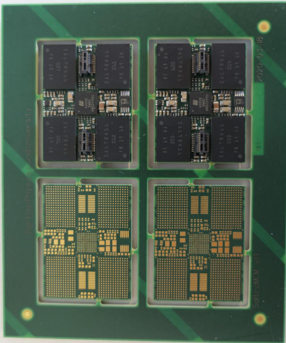
Top and bottom of an MCM panel board with two MCM-boards version 2 mounted
