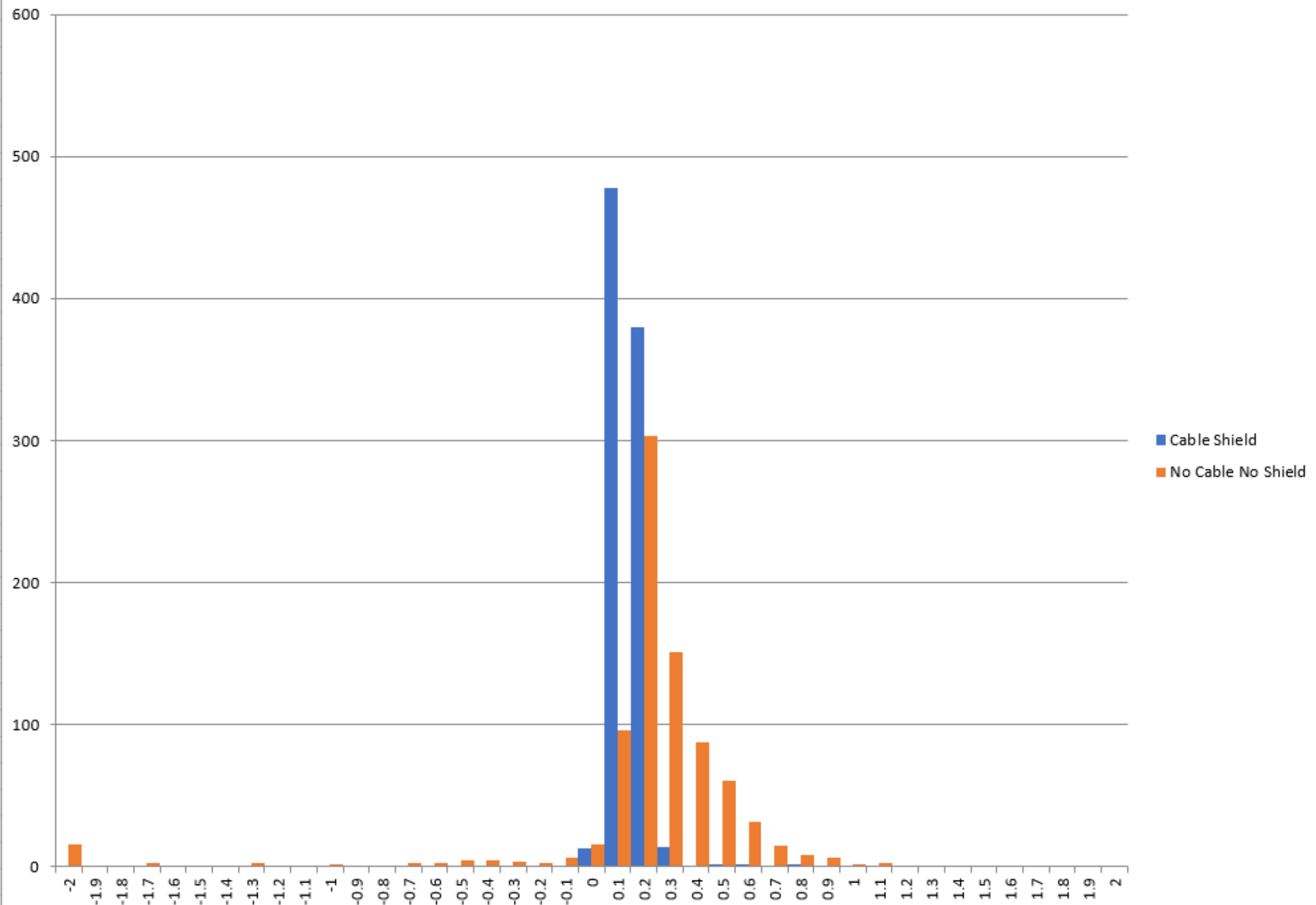
Crosstalk (%) Distribution GUI 493 Normal Gain
