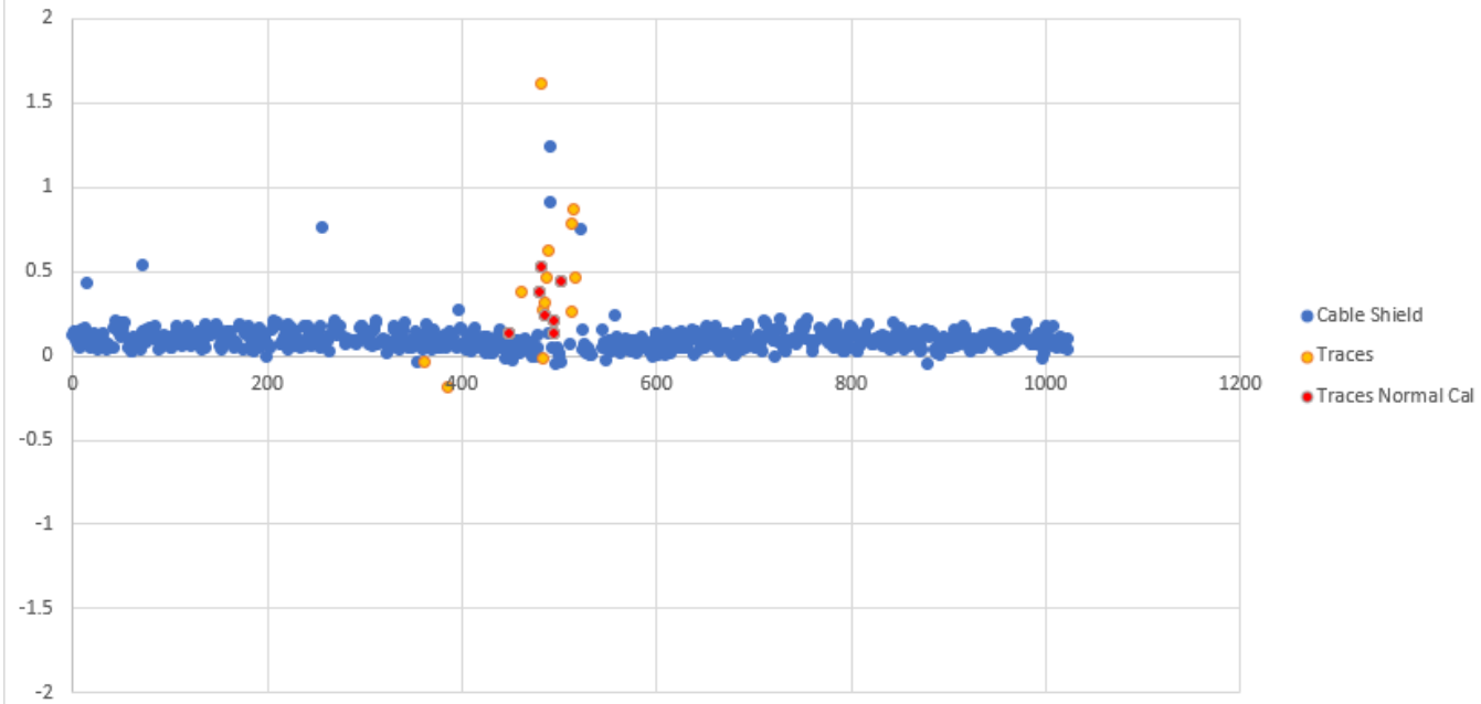
Cable Shield (Crosstalk vs KPiX)
