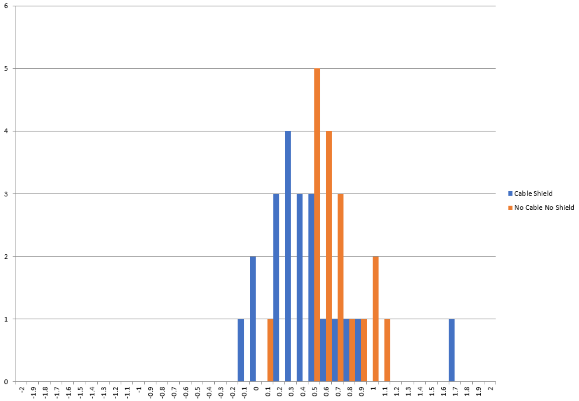
Crosstalk (%) Distribution GUI 493 Traces
