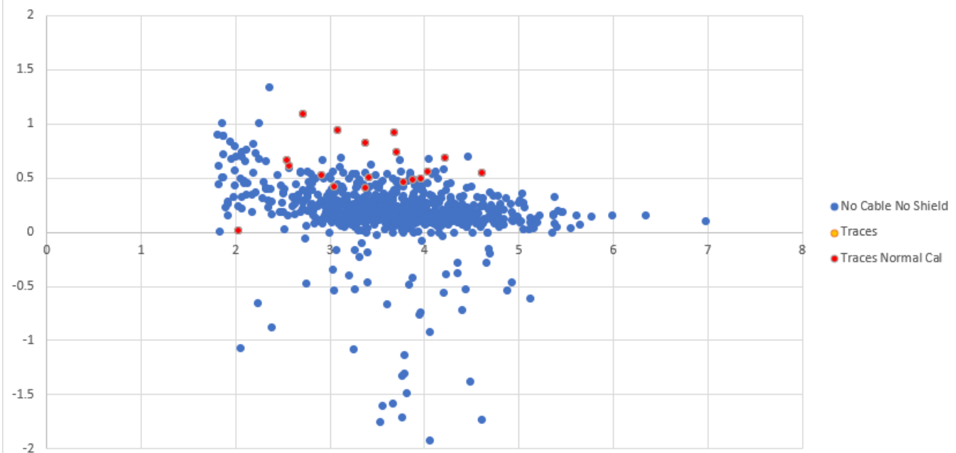
No Cable No Shield (Crosstalk vs Cal)
