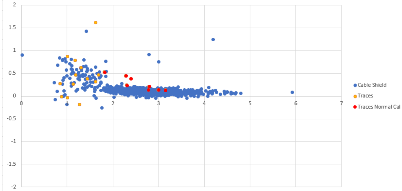
Cable Shield (Crosstalk vs Cal)
