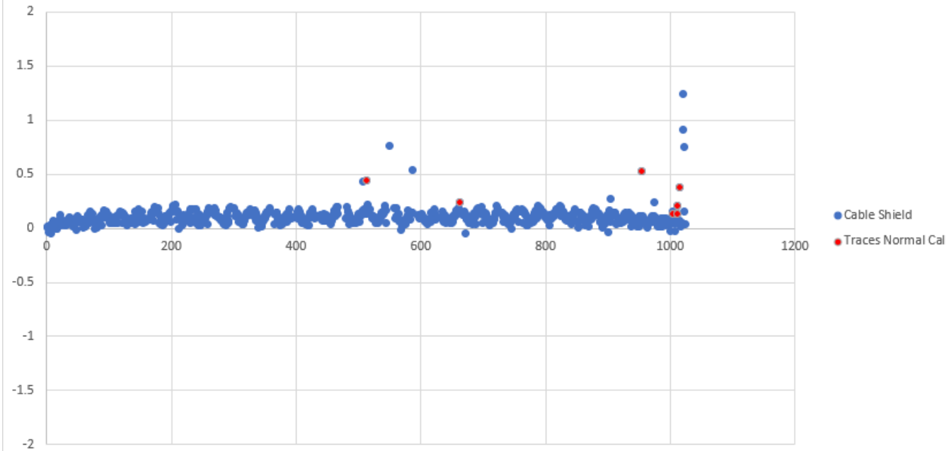
Cable Shield (Crosstalk vs HAMA)
