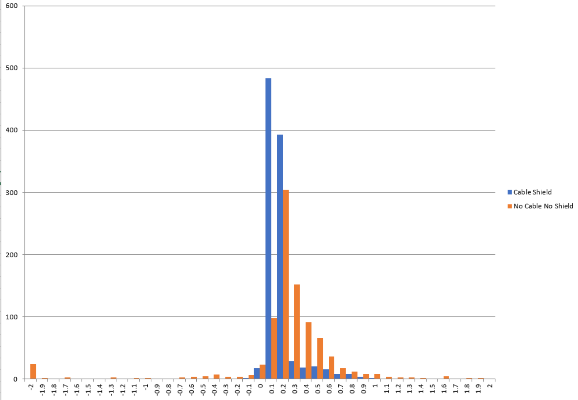
Crosstalk (%) Distribution GUI 493 All Channels
