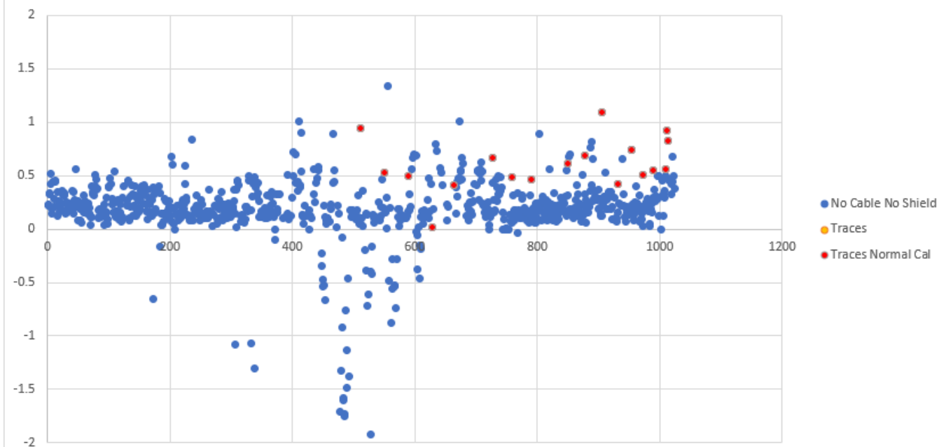
No Cable No Shield (Crosstalk vs HAMA)
