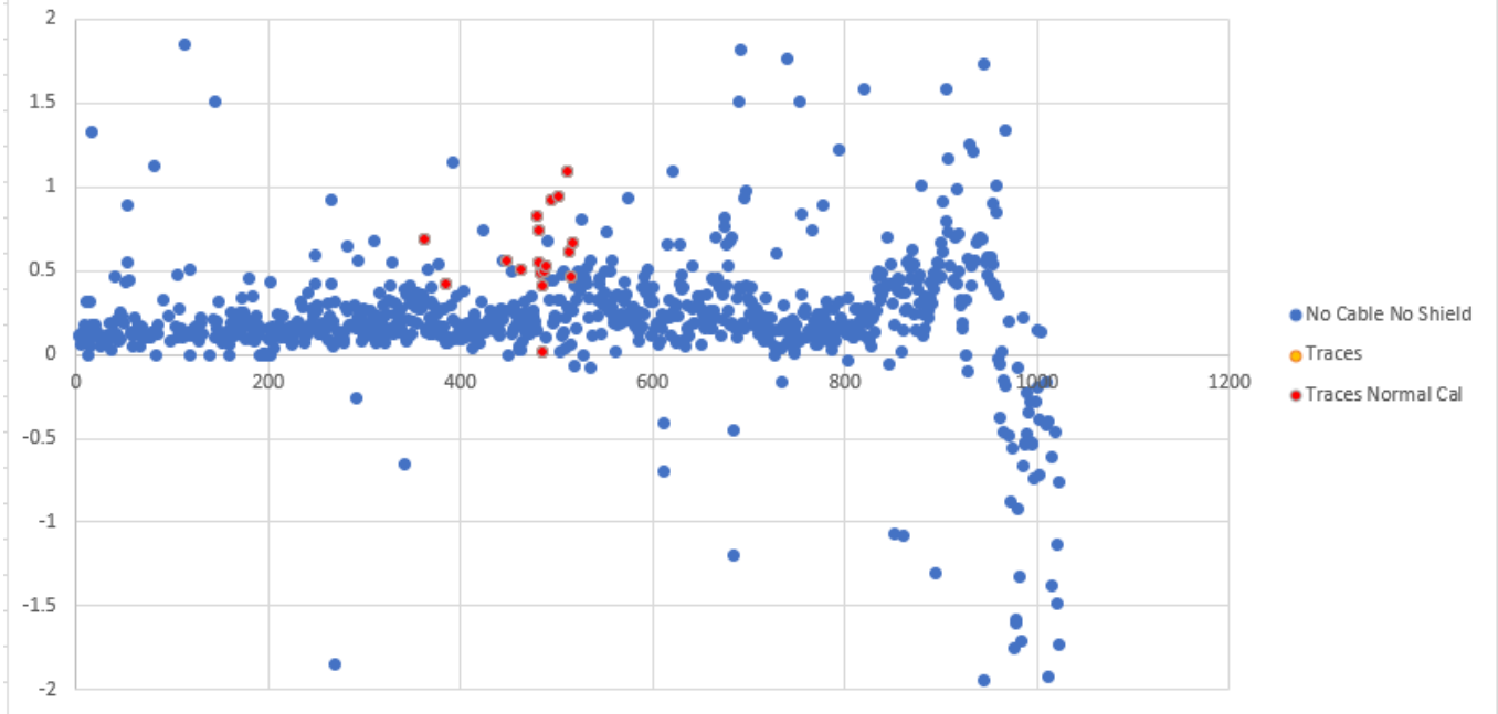
No Cable No Shield (Crosstalk vs KPiX)
