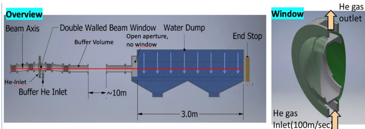
Figure 2: Layout of water based photon dump.
