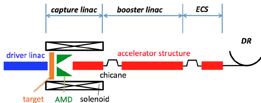
Fig. 1: Schematic of the e-driven ILC positron source. Positrons generated in target are captured by capture linac. After removing electrons by chicane, positrons are boosted up to 5 GeV and injected to the DR via the ECS.
