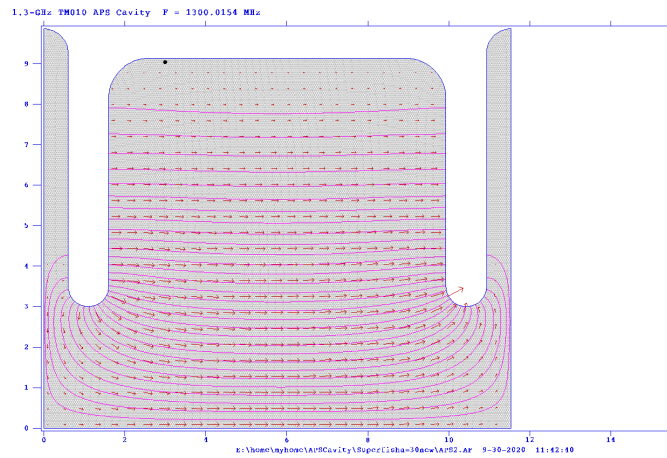
Fig. 6: Field map of APS cavity calculated by
