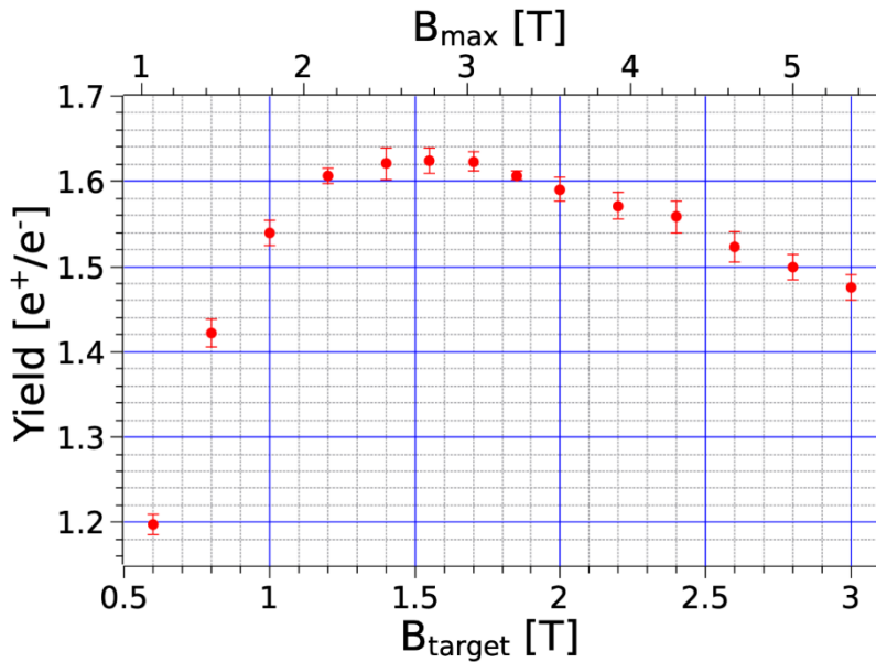
Fig. 3 Expected e^+ yield depending on the B-Field at the target exit and the peak field inside the solenoid.
