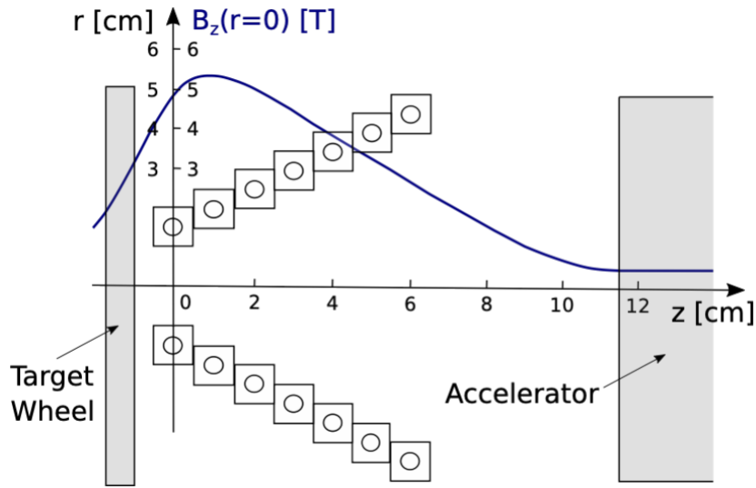
Fig. 2 OMD: Schematic layout of the water cooled windings of the pulsed, conical solenoid together with the magnetic field.
