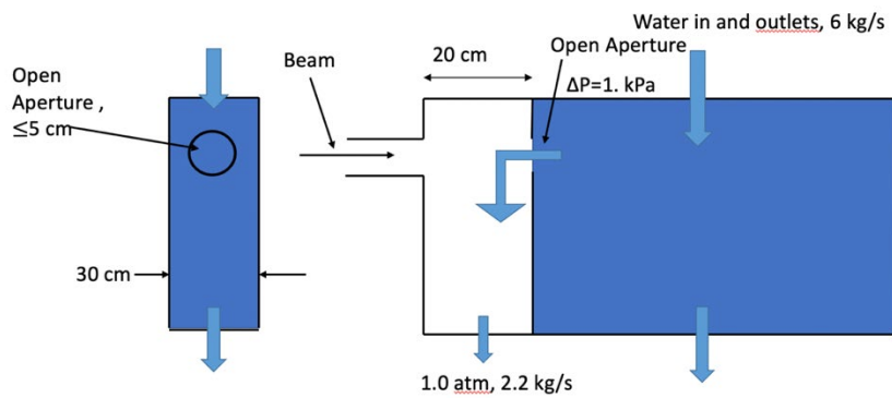
Figure 3: Concept of open-window water dump.
