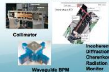
Waveguide BPM
