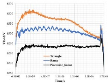
Induction kicker pulsar for CLIC DR
