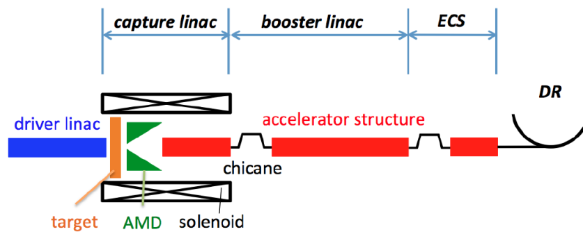
Figure 1: Schematic of the e-driven ILC positron source. Positrons generated in target are captured by capture linac. After removing electrons by chicane, positrons are boosted up to 5 GeV and injected to the DR via the ECS.
