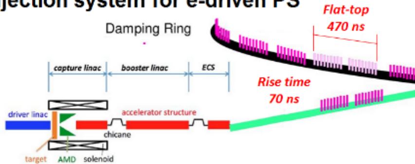
Injection system for e-driven PS
