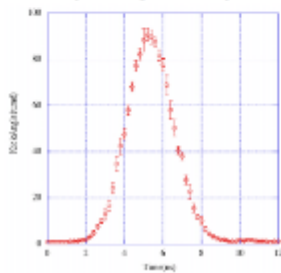
Beam test in ATF DR (5kV pulsar)
