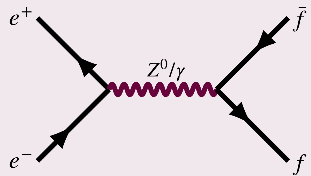
Figure 1 Feynman diagram for fermion pair production at e^+e^- collision through Z^0/\gamma at Leading Order. Studies of t\bar{t} / b\bar{b} / c\bar{c} pair production are being conducted.
