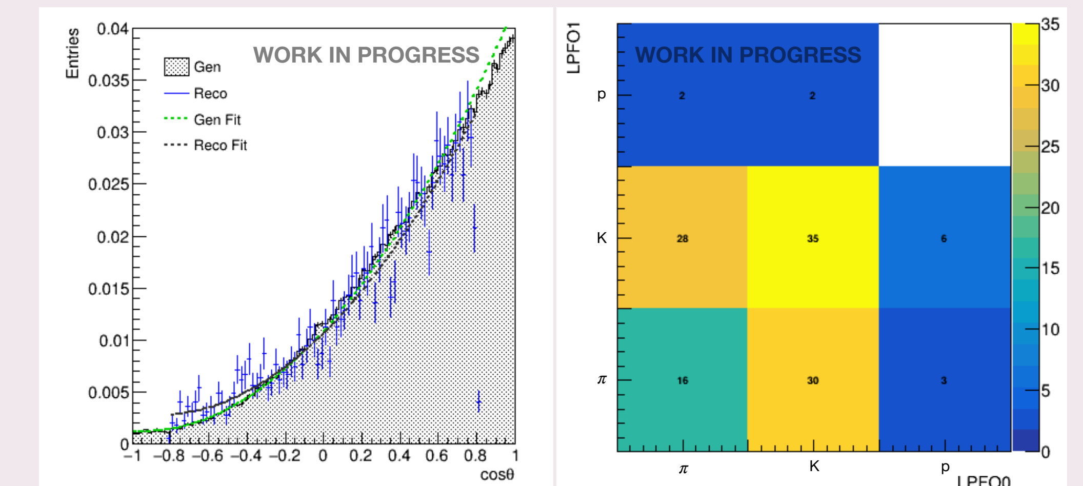
Figure 9 Polar angle distribution of LPFOs after the selection (left) and true PDG information of LPFO with wrongly reconstructed charge (right). Note that due to the TPC detector acceptance (# of hits), there is little to no sensitivity at the forward region ( |\cos\theta| > 0.8 )
