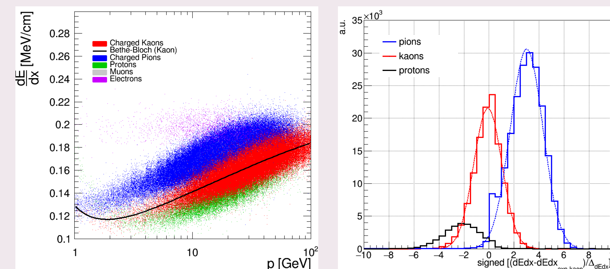
Figure 6 dE/dx vs p distribution (left) and dE/dx distance calculated by eq (2) for e^+e^- \rightarrow s\bar{s} process. The dominant backgrounds are pions and protons.
