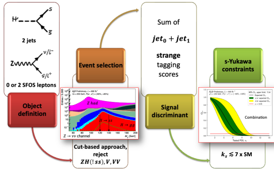
(b) Flow chart of the Zh with h \rightarrow s\bar{s} analysis.
